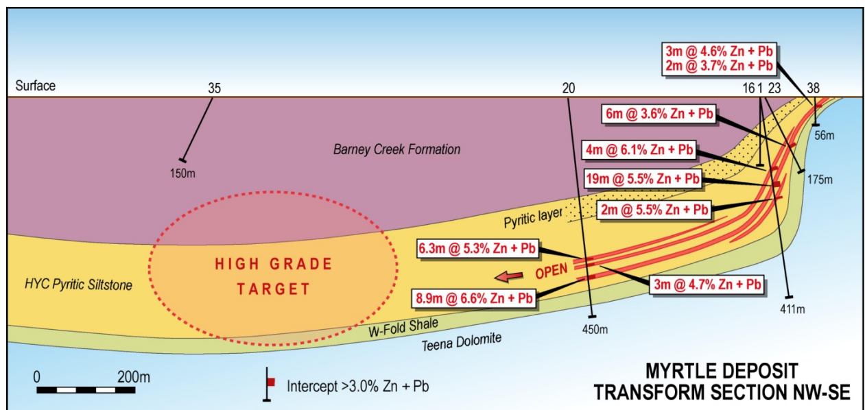
Figure 3: Myrtle Drill Cross Section (section line as per Figure 2 above)
