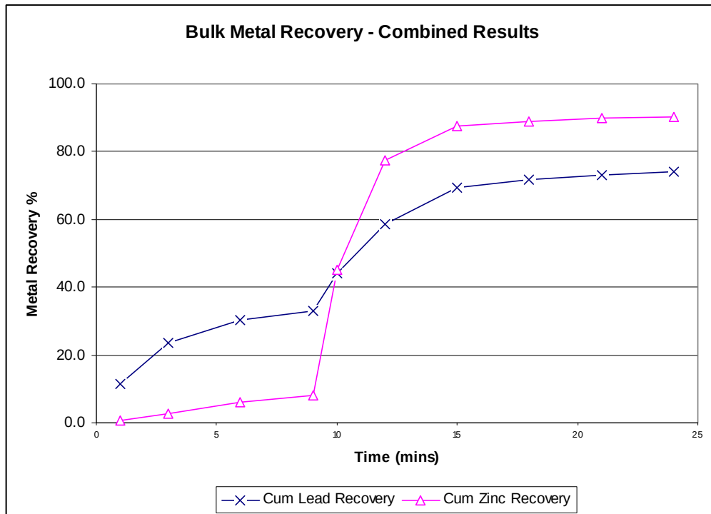
Figure 4: Recovery vs. Time Graph
