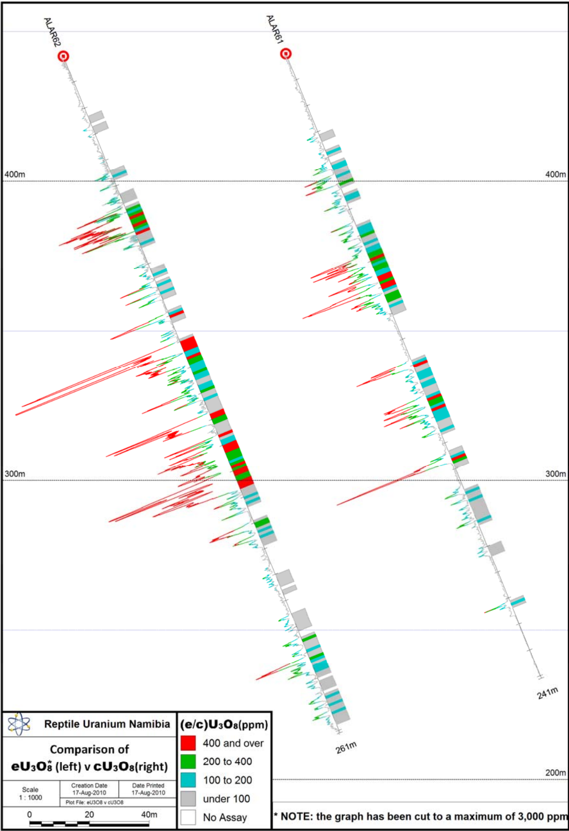
Figure 5: Tubas Alaskite Reconnaissance Line 2 Holes ALAR61 and ALAR62. Comparison of chemical assays (cU 3 O 8 ) v gamma probe results (eU 3 O 8 ) which are top cut to 3,000 ppm eU 3 O 8
