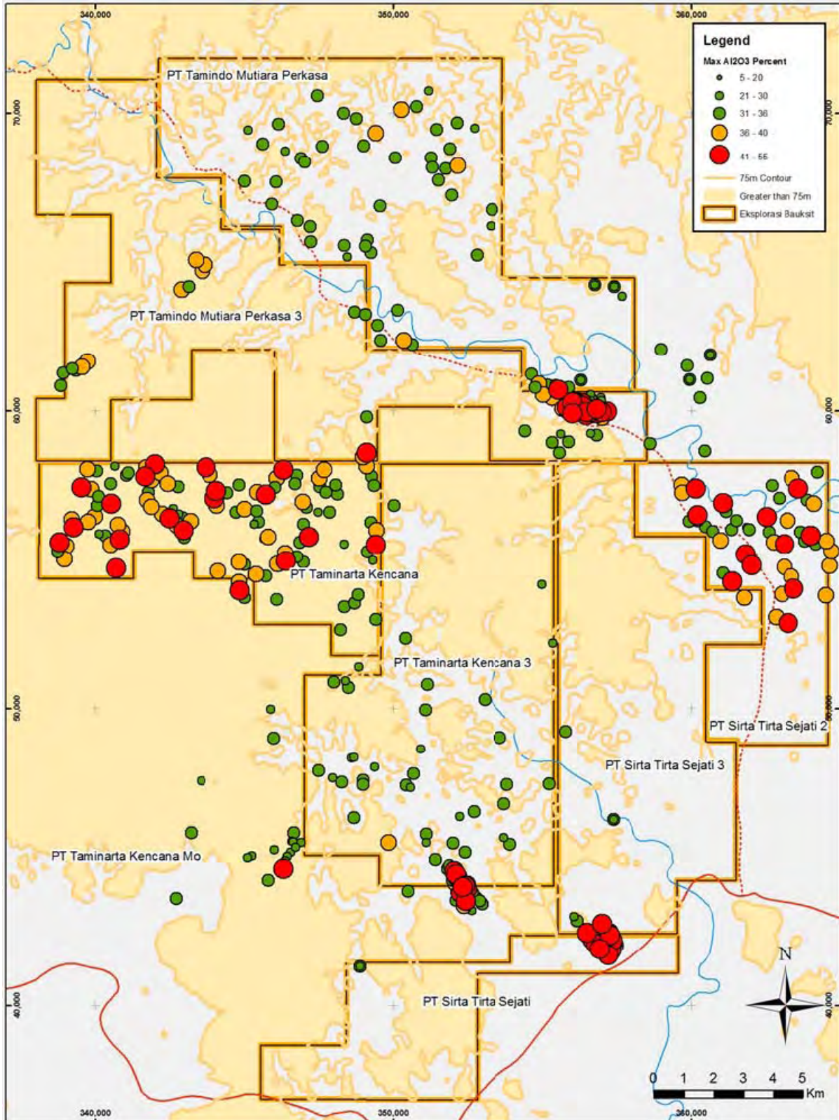
Figure 3. Landak Project Tenure and Reconnaissance Sampling Al 2 O 3 Grade Map
