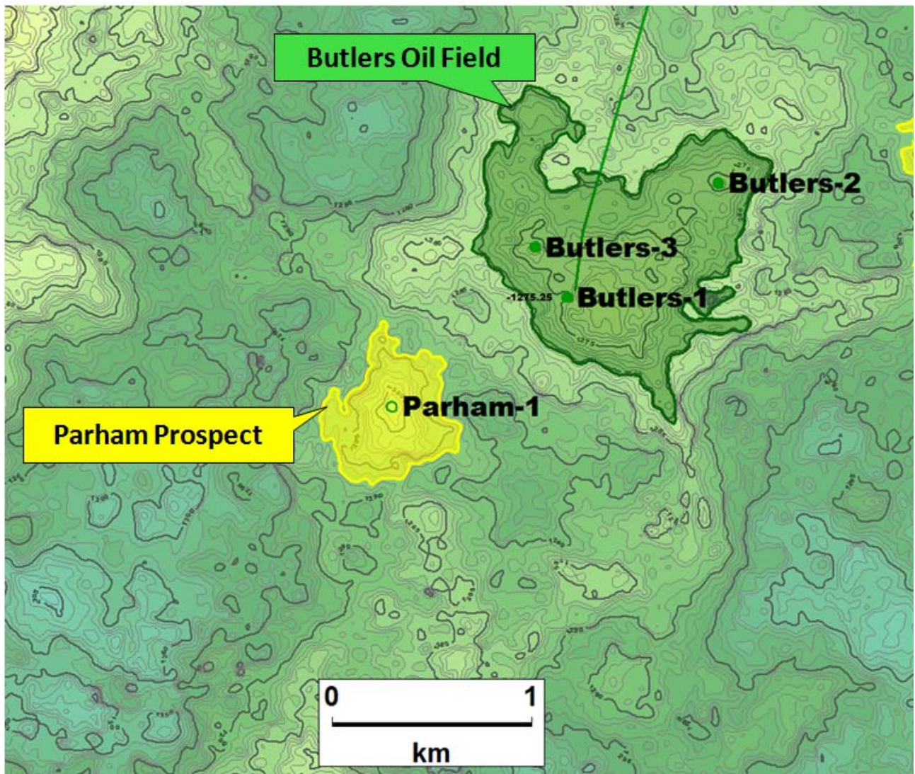
Parham Prospect Map with Parham-1 Well Location and Butlers Oil Field.
