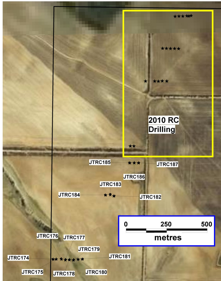
Figure 1. Location of 2011 Jamieson Tank drillholes
