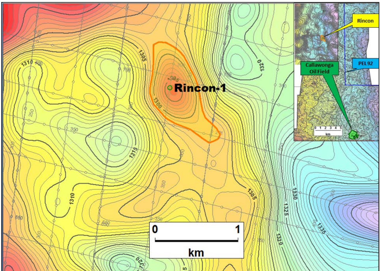
Rincon Prospect Map with Rincon-1 Well Location and nearby Callawonga Oil Field.
