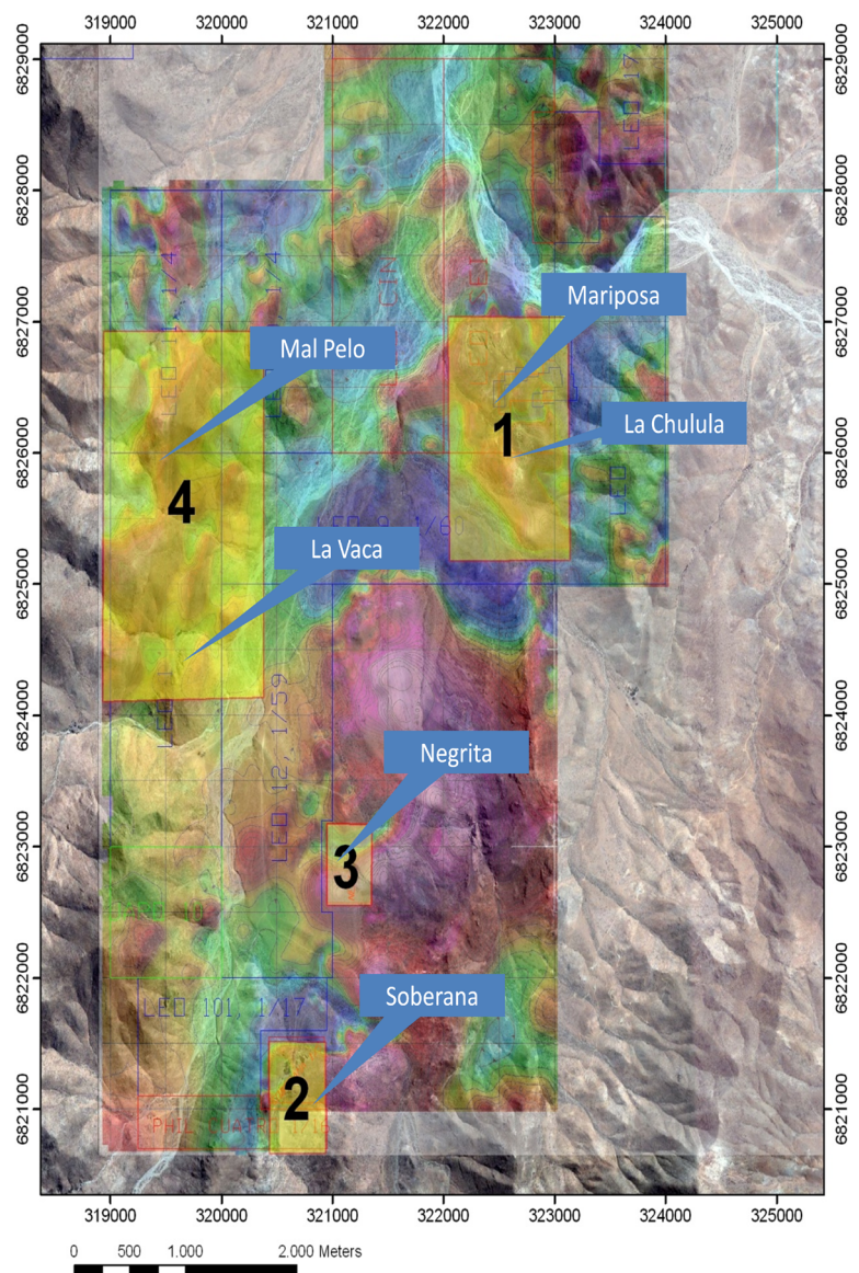
Figure 1: Aerial photo showing the Southern Region of the Harper Geological District and the prospective areas identified for high resolution ground magnetic survey highlighted in yellow and ranked in execution order.
