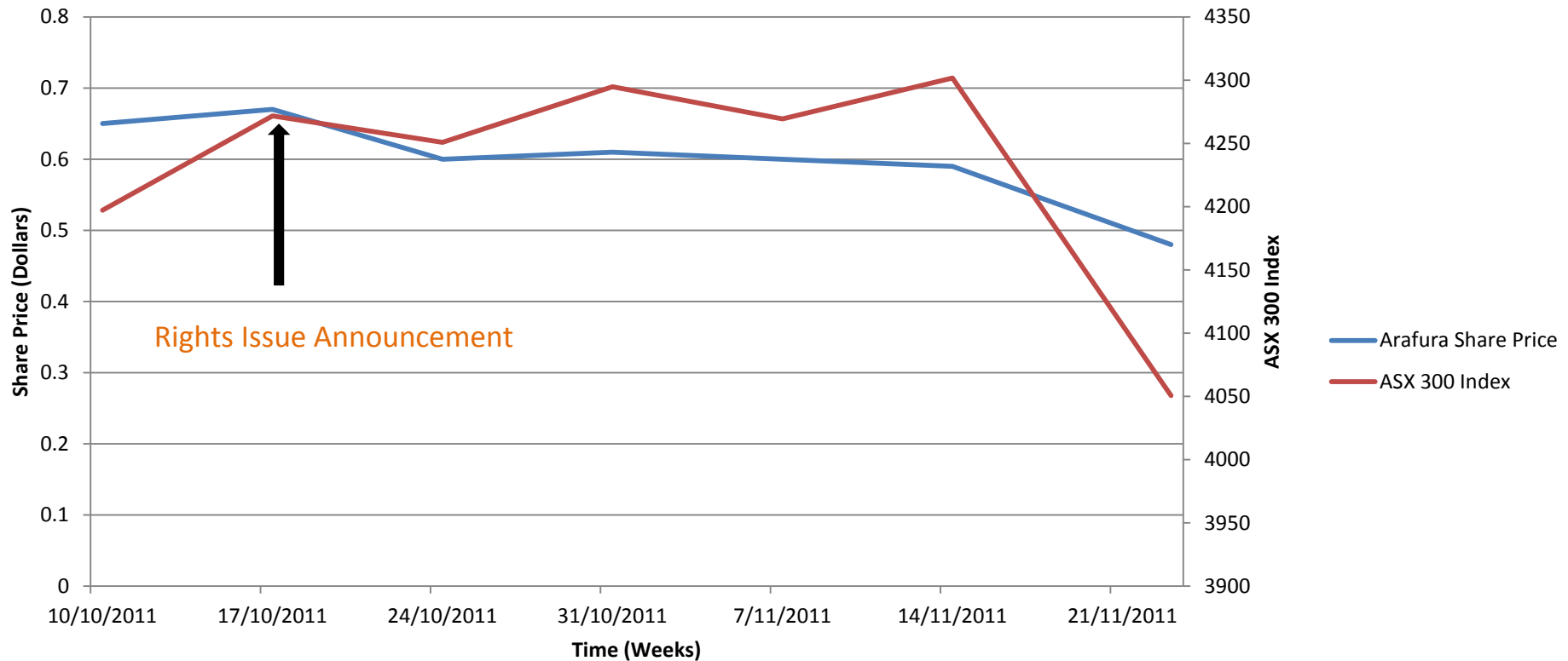
Arafura Share Price vs ASX 300 Index
