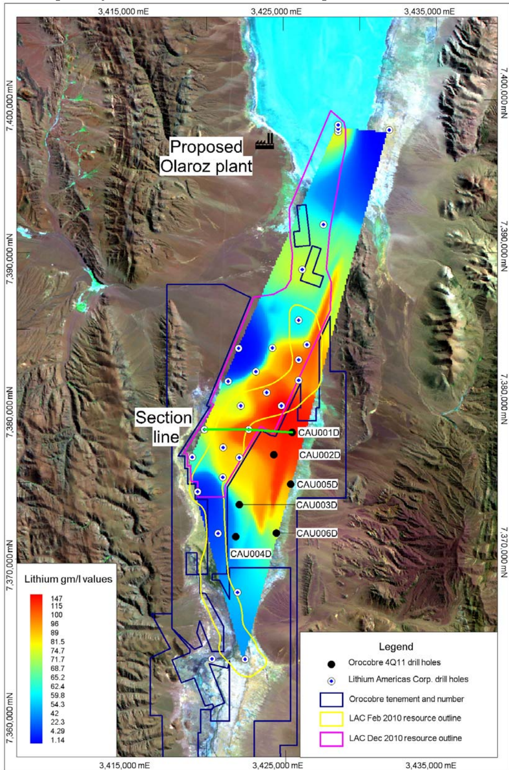
Figure 2 Drill hole locations over an image of lithium gram-metre/litre (averaged g/l lithium values multiplied by the thickness in metres over which they occur) values compiled from publicly released Lithium Americas Corp. data
