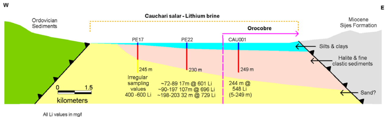
Figure 3: East-west interpretive cross section, looking north through the Cauchari salar, based on Orocobre CAU001D and publicly available Lithium Americas Corp data
