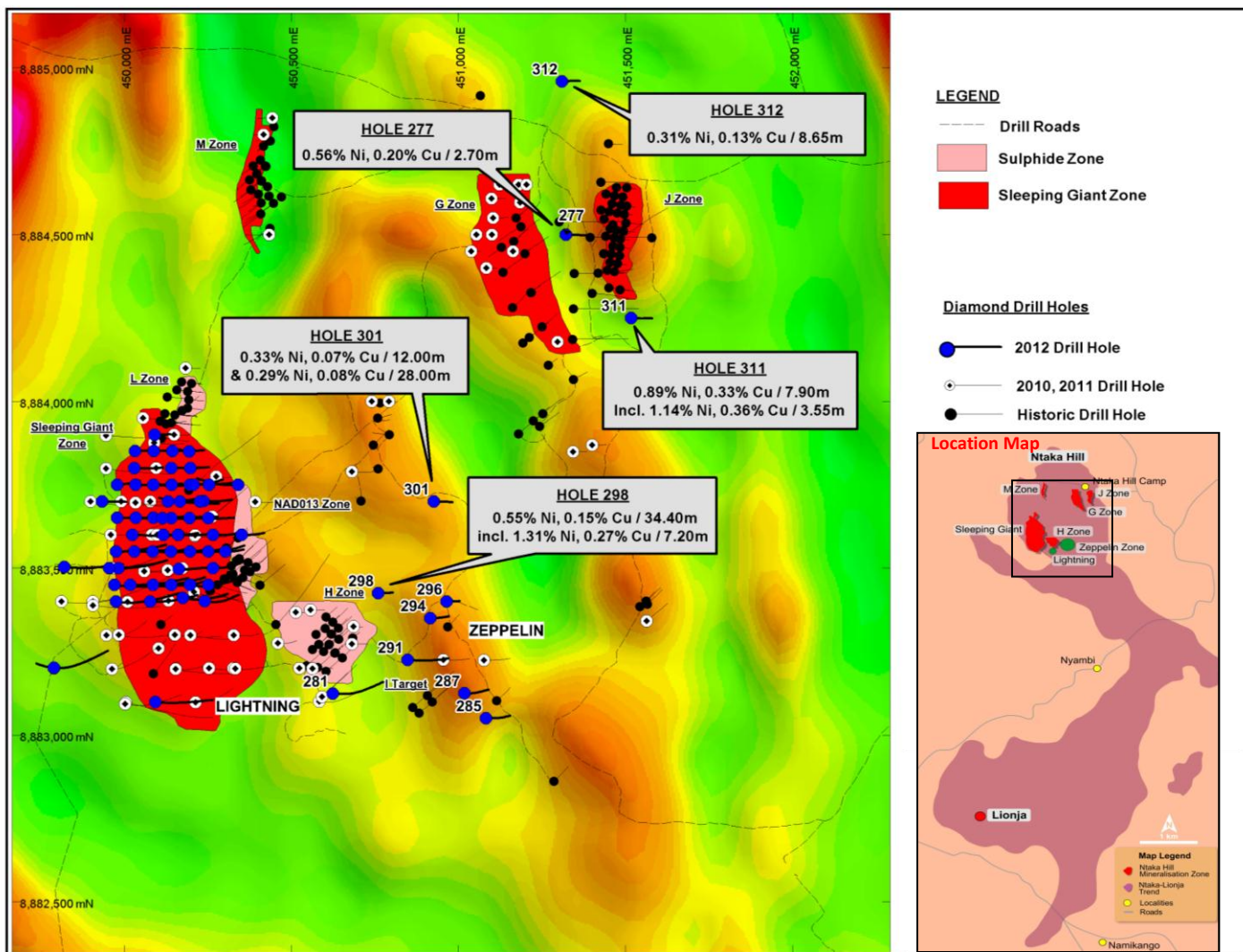
Figure 1: Ntaka Hill Geochemical Exploration Target Intersections on Reduced to Pole (RTP) magnetics
