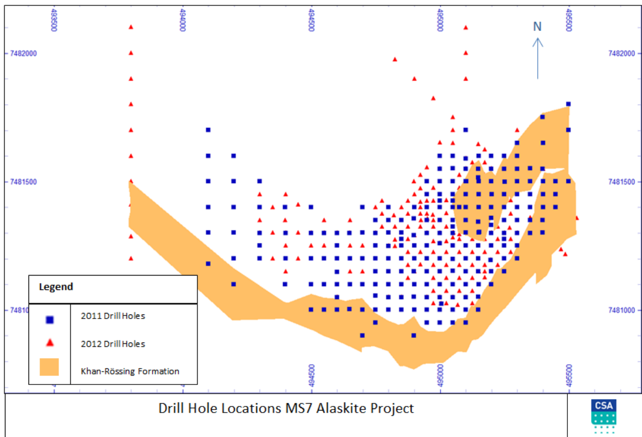
Figure 2: MS7 Drill Holes December 2011 and November 2012
