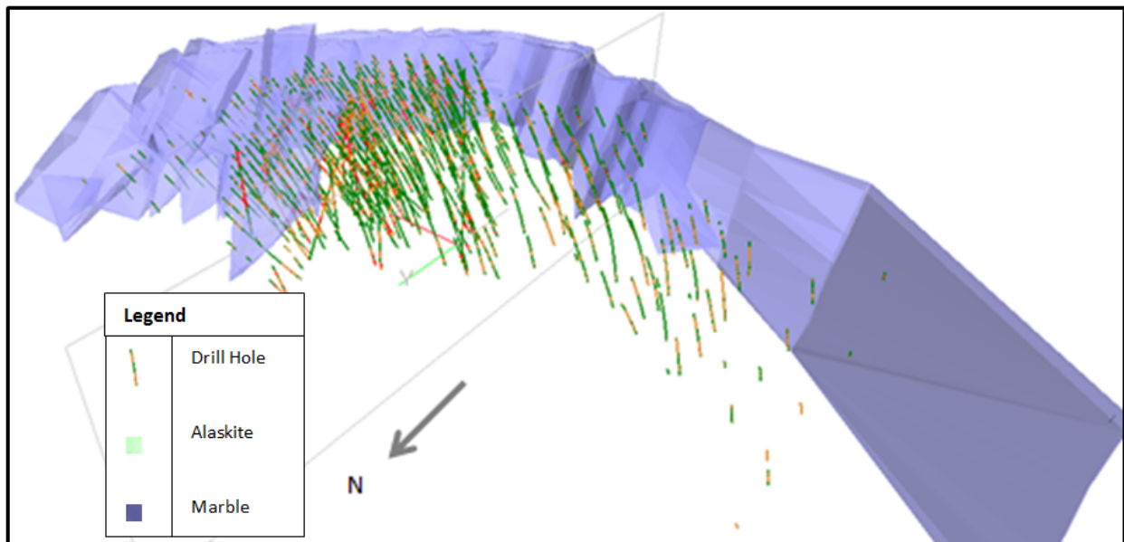
Figure 3: MS7 Drill Holes in Relation to the Marble Country Unit
