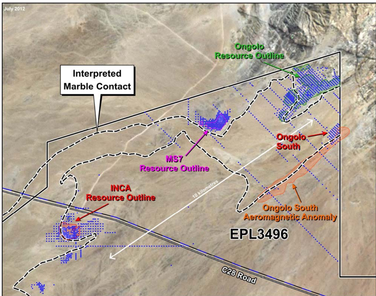
Figure 1: Omaha Project Resource Outlines and Drilling – Ongolo, MS7 and INCA Deposits
