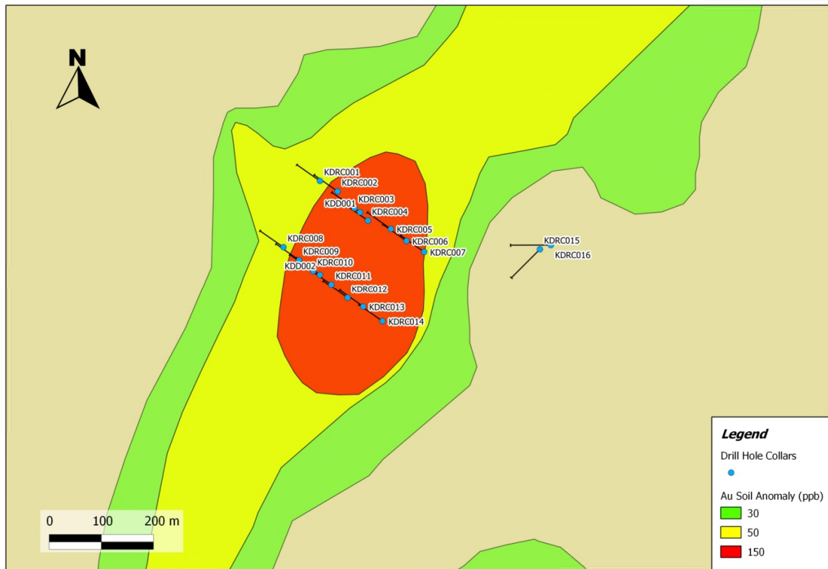
Figure 4: First pass RC drilling fences on a central soil anomaly.
