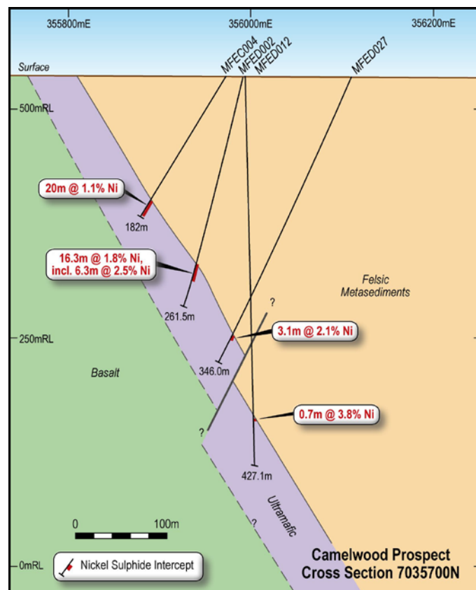
Figure 6: Camelwood Drill Cross Section 7035700N
