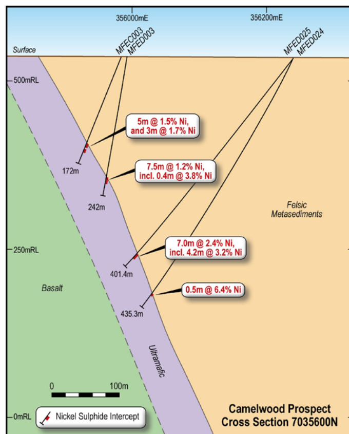
Figure 5: Camelwood Drill Cross Section 7035600N
