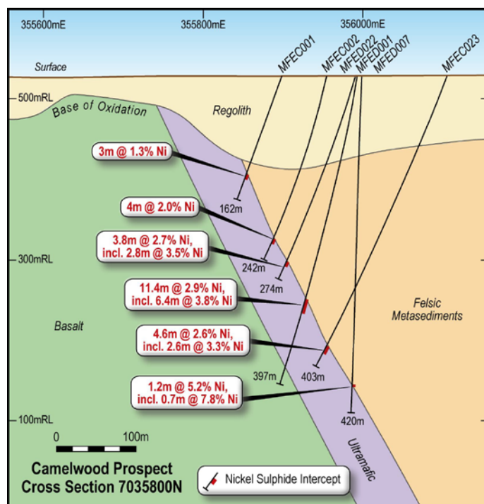
Figure 7: Camelwood Drill Cross Section 7035800N
