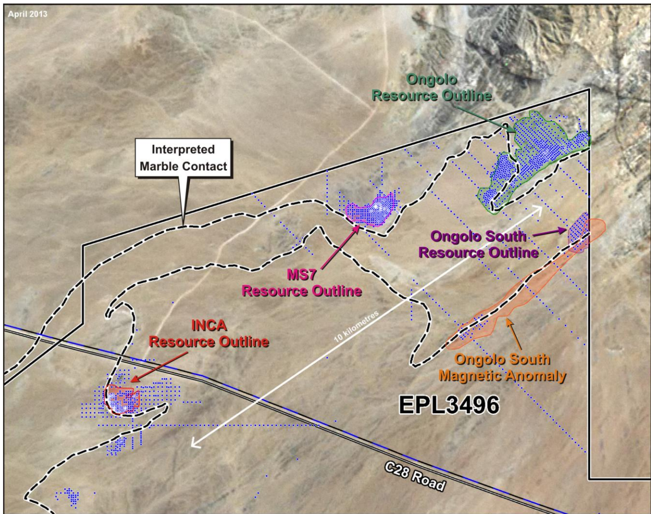
Figure 1: Locality Map showing Omahola Project Resource Outlines
