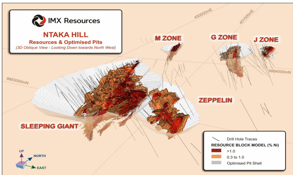
Figure 2. Ntaka Hill global resource, three-dimensional view of the block model
