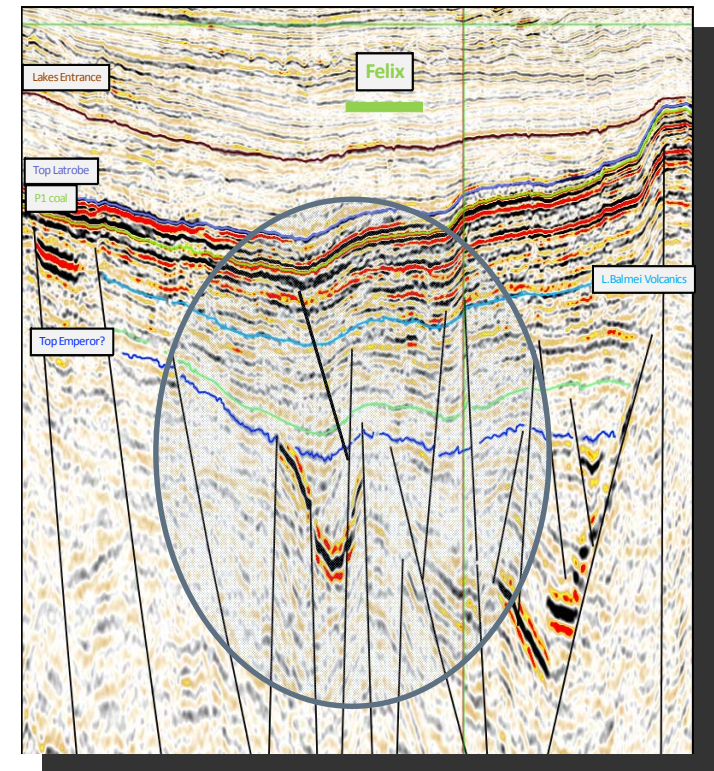
Seismic line through Felix from the new reprocessed data
