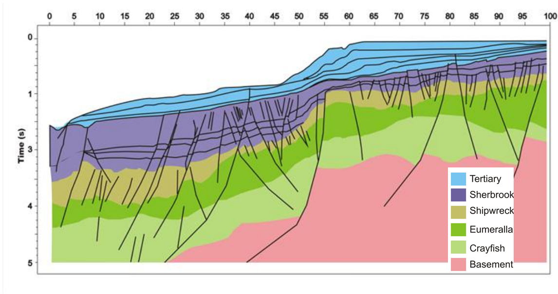
Figure 12: Schematic cross section through T/49P
