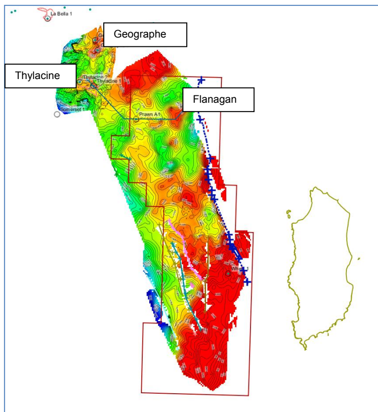
Figure 11: Time structure base seal
