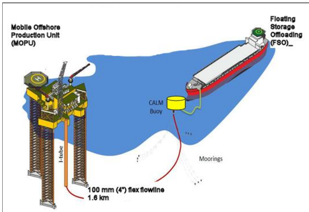
Figure 3: Schematic illustration of the West Seahorse development
