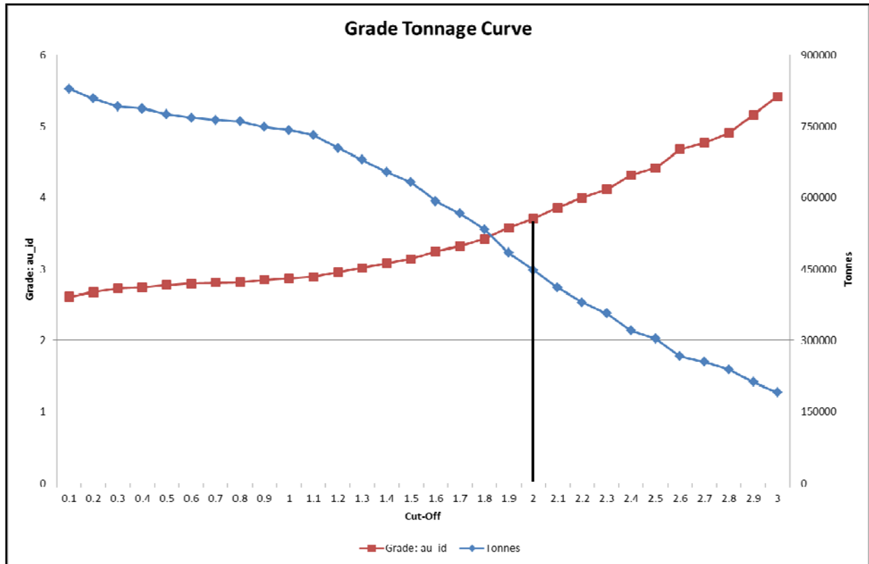
Figure 2: Tonnage Grade Curve –September 2013 Golden Wings Resource
