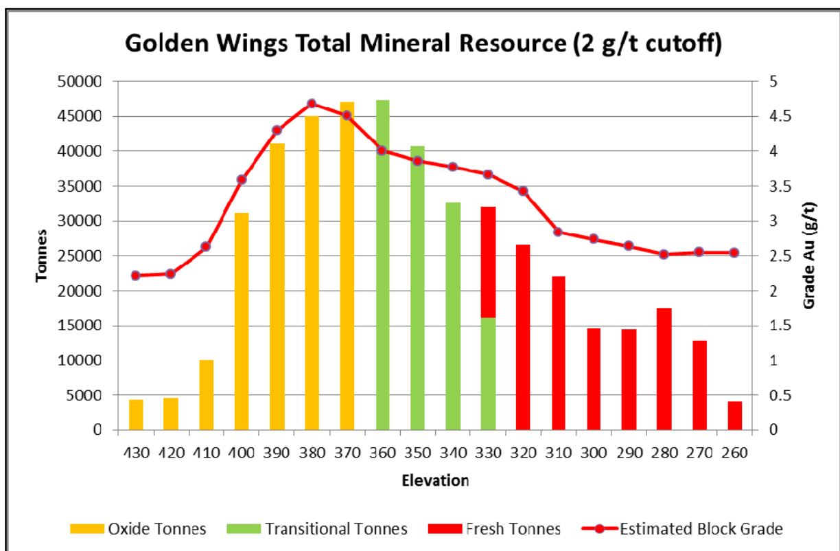
Figure 3: Golden Wings Resource per 10m bench, showing grade and bench tonnage
