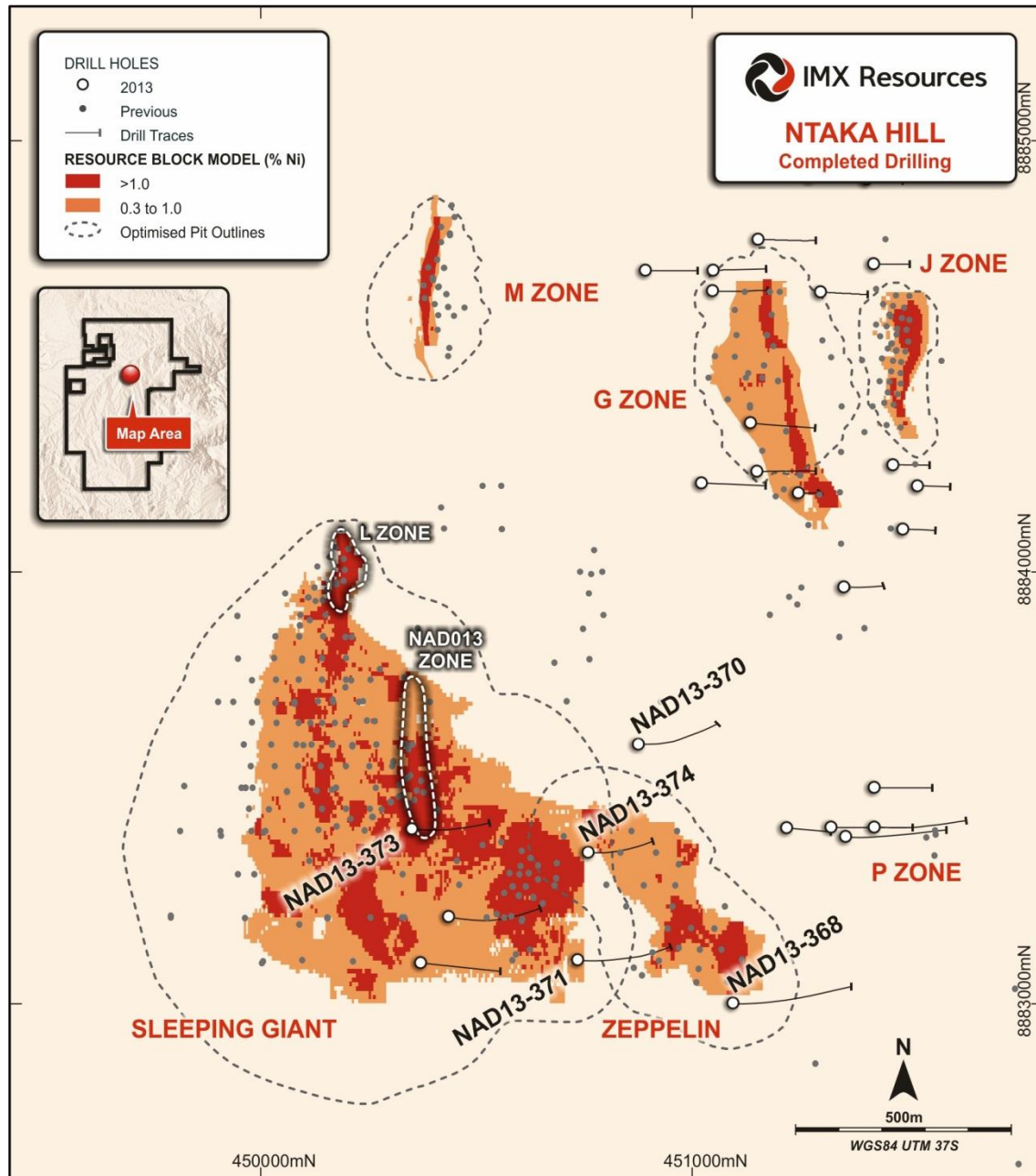
Figure 2: Initial Drill Hole Collar Locations
