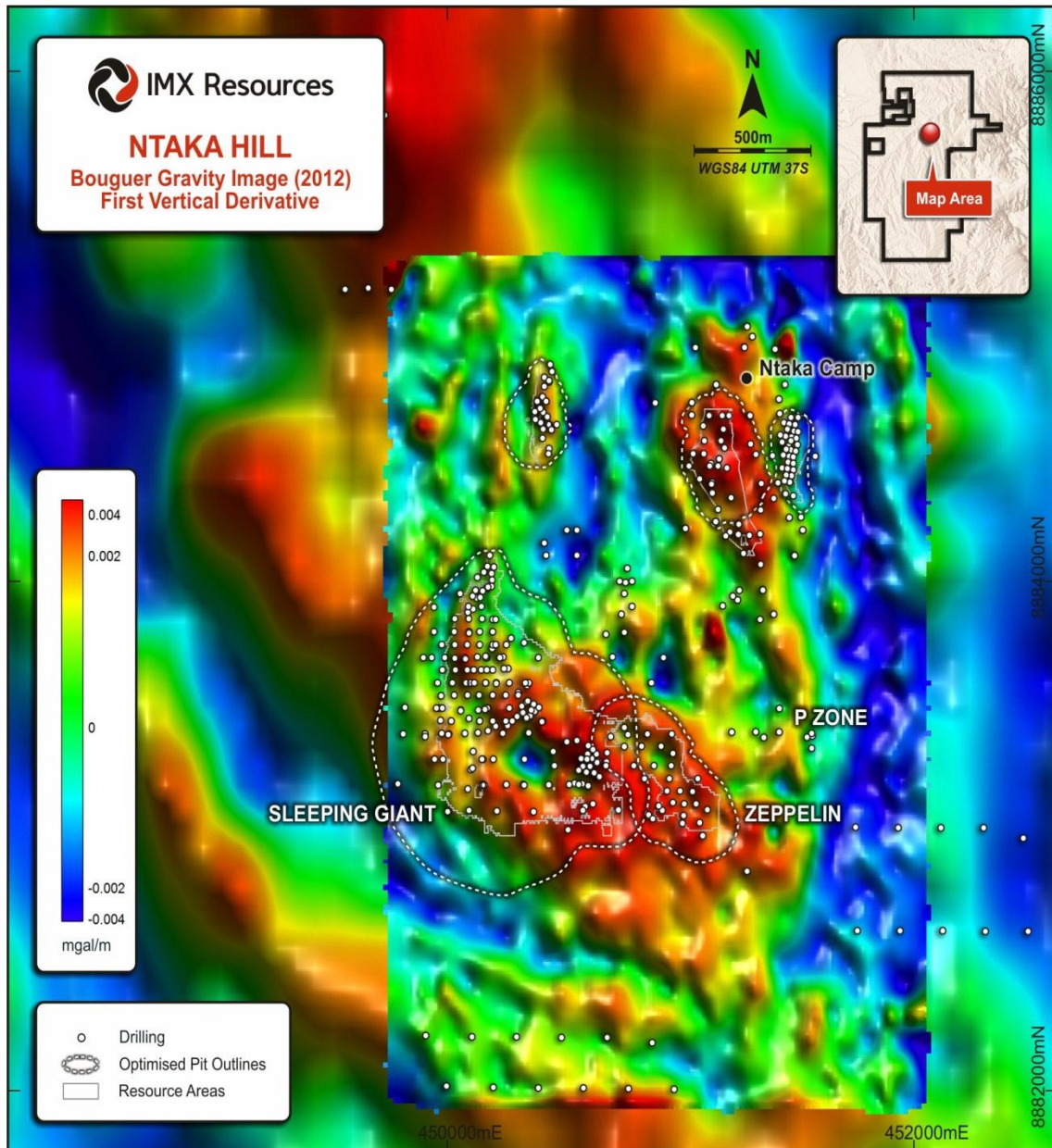
Figure 1: Regional one VD gravity image
