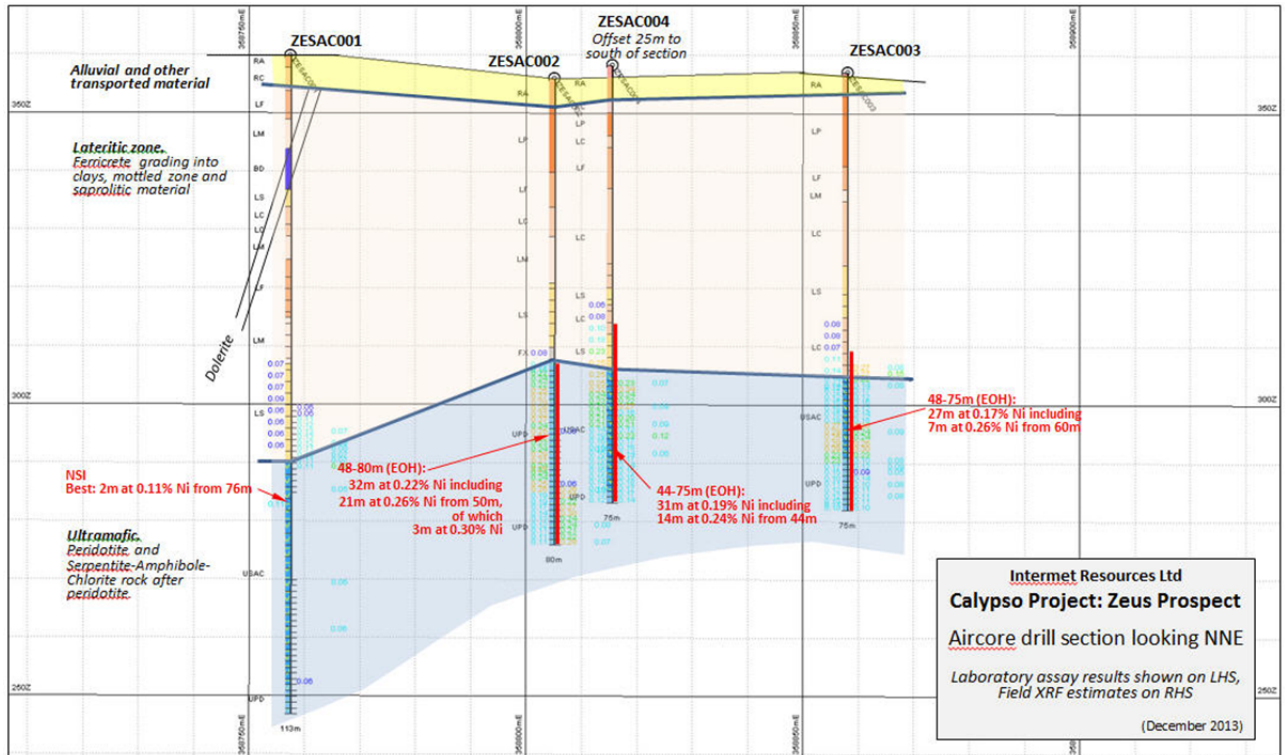
Figure 2. Zeus prospect aircore drill section looking NNE
