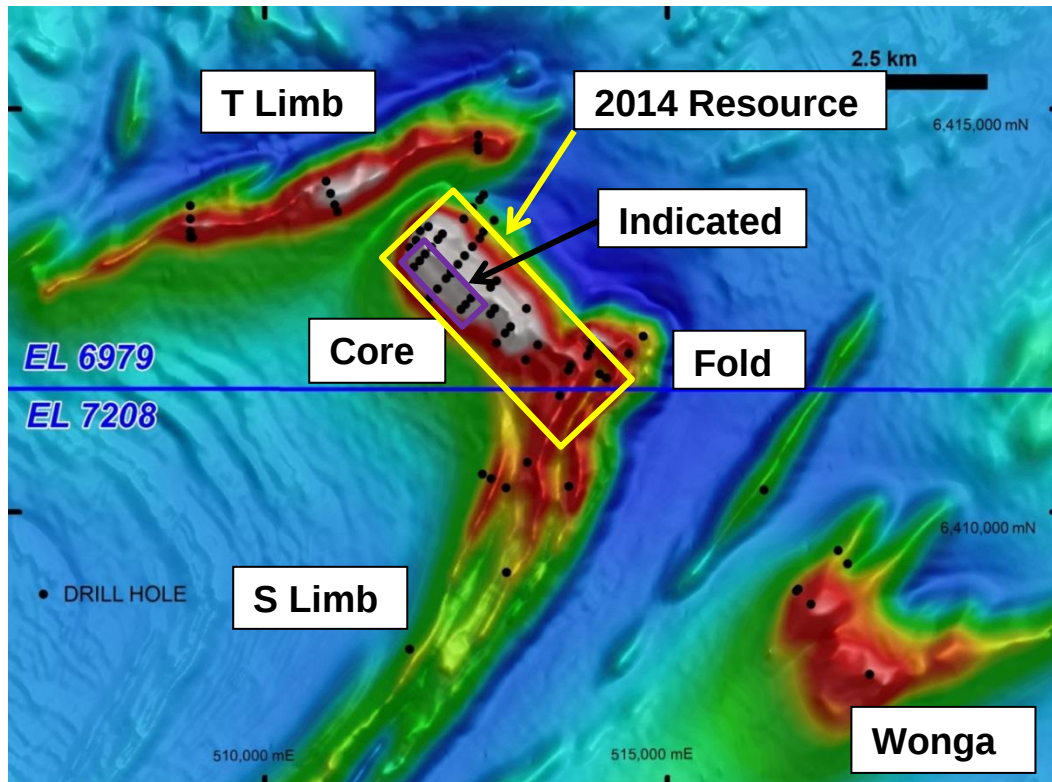
Figure 1 Airborne Magnetic Data and Prospect Areas
