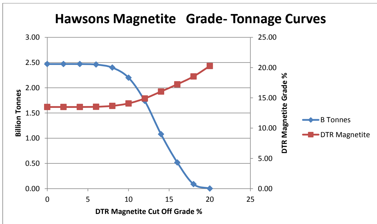
Figure 12 Hawsons Magnetite Project Grade – Tonnage Curves
