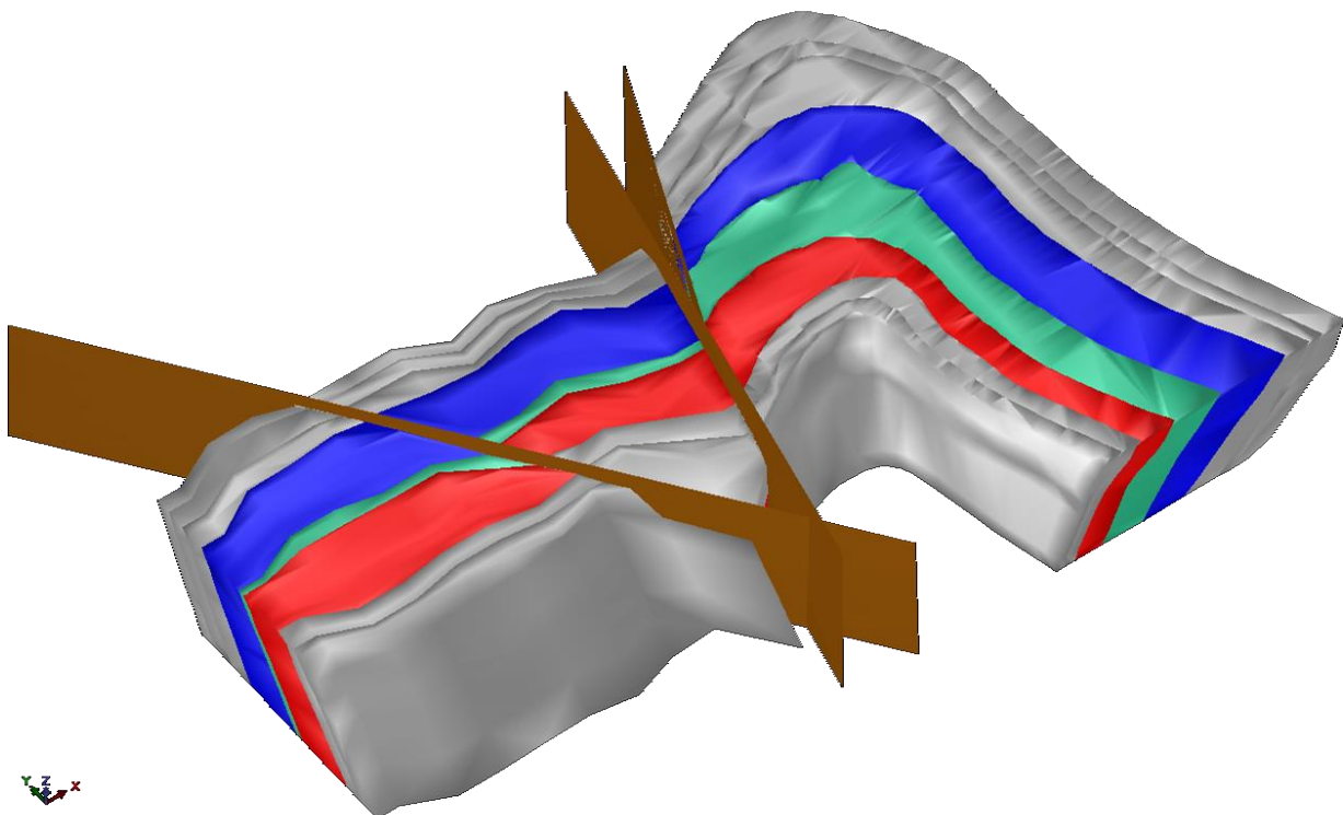
Figure 4 Core-Fold Prospects 3D Geology
