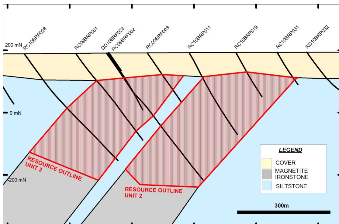
Figure 2 Core Area Schematic Cross Section
