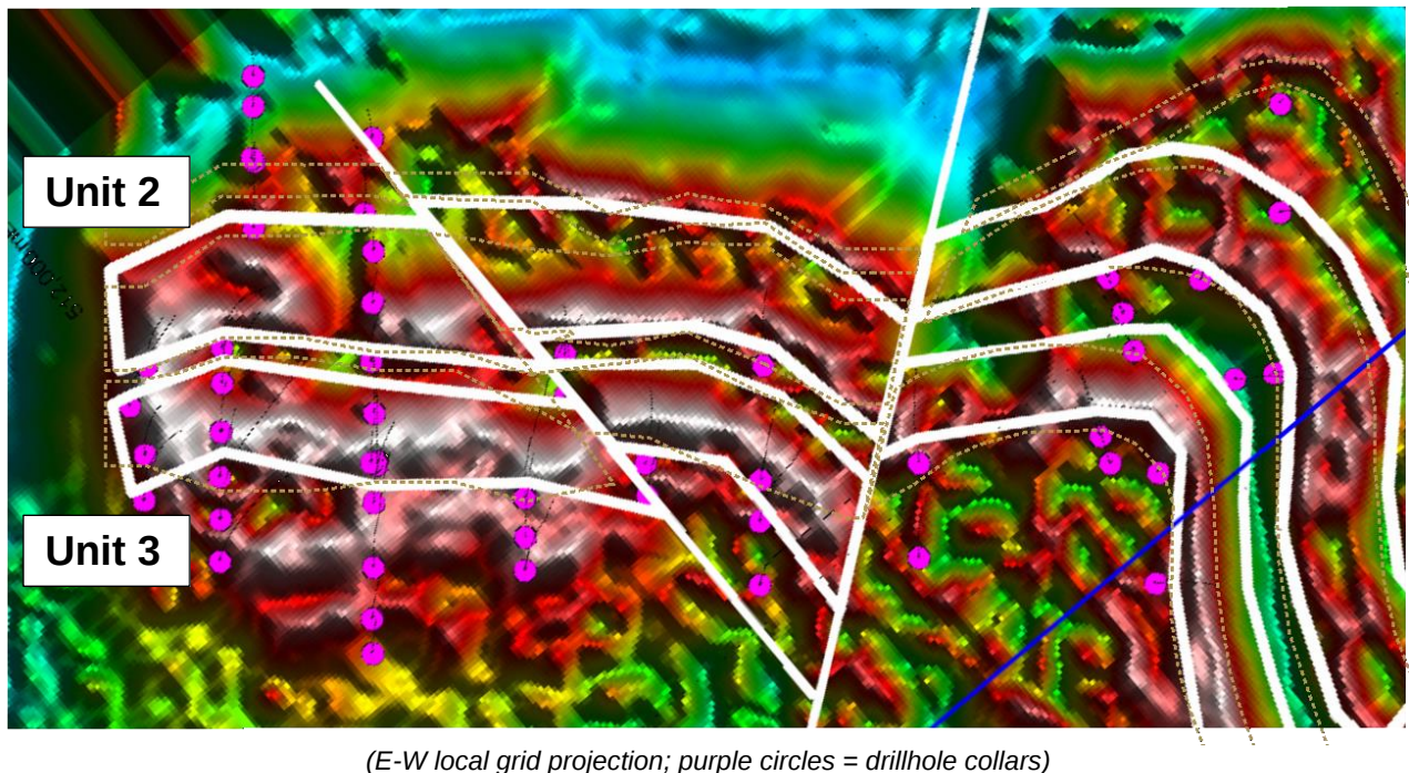
Figure 3 Core-Fold Prospects Geological Model & Ground Magnetic Interpretation
