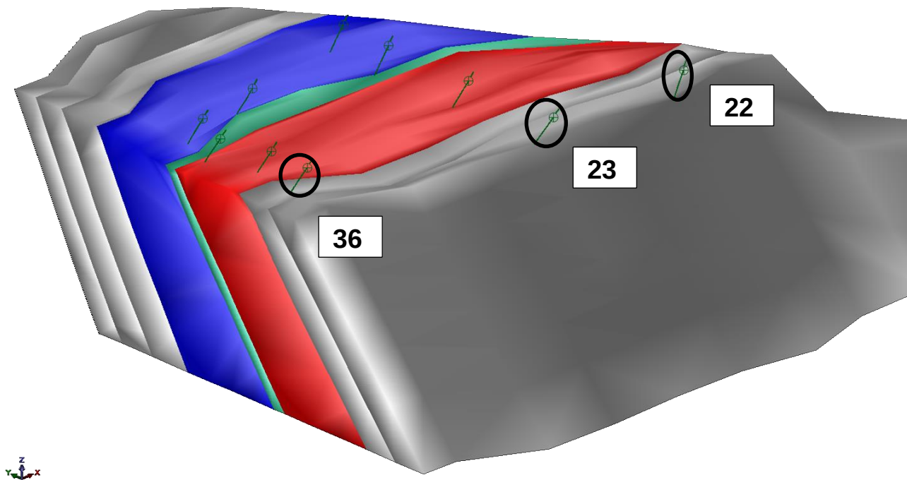
Figure 5 Core West Deposit Geological Delineation of Units for Detailed Study
