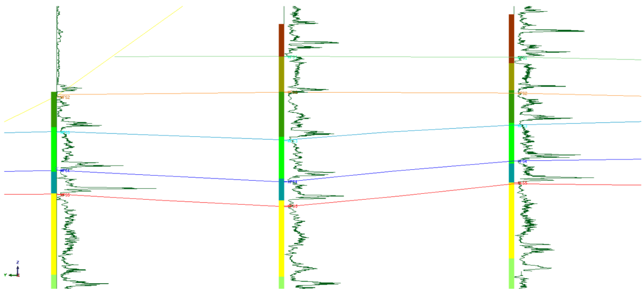
Figure 7 Downhole Magnetic Susceptibility Data with CAP Interpretation & MFS Interpretation
