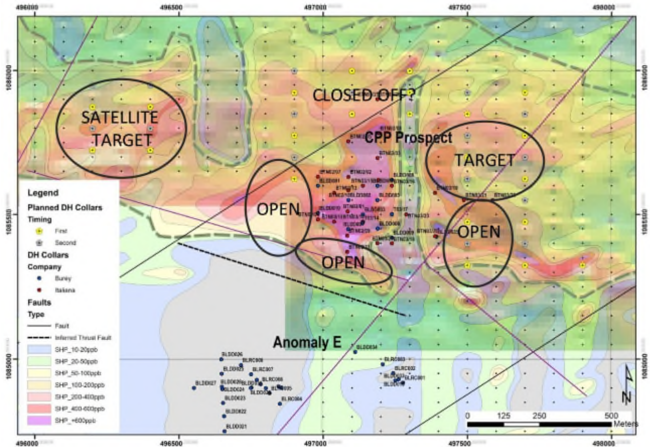
Figure 2: Location of drilling targets confirmed by MSA at the CPP (Balatindi)
