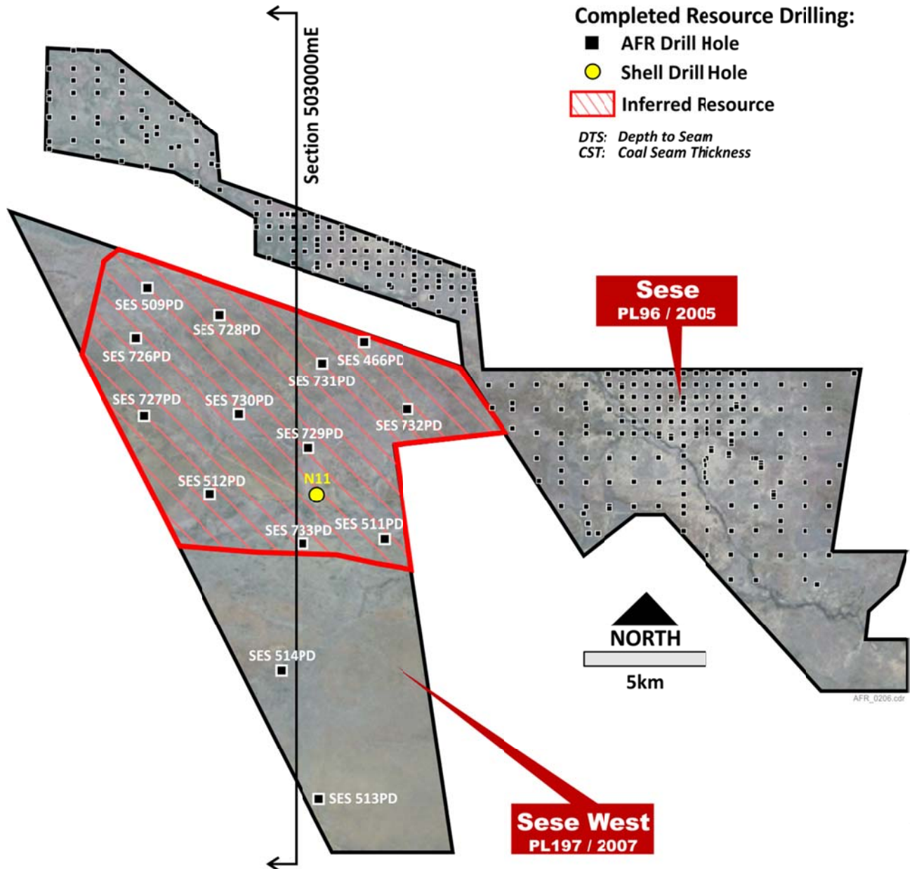
Diagram 2 – Plan showing Sese West drill hole collar locations and proximity to Sese coal deposit
