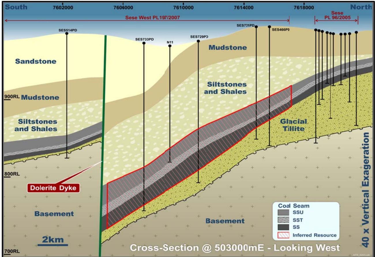
Diagram 3 – Cross-Section through Sese West Inferred Resource and showing up-dip continuation into African Energy’s nearby Sese coal deposit
