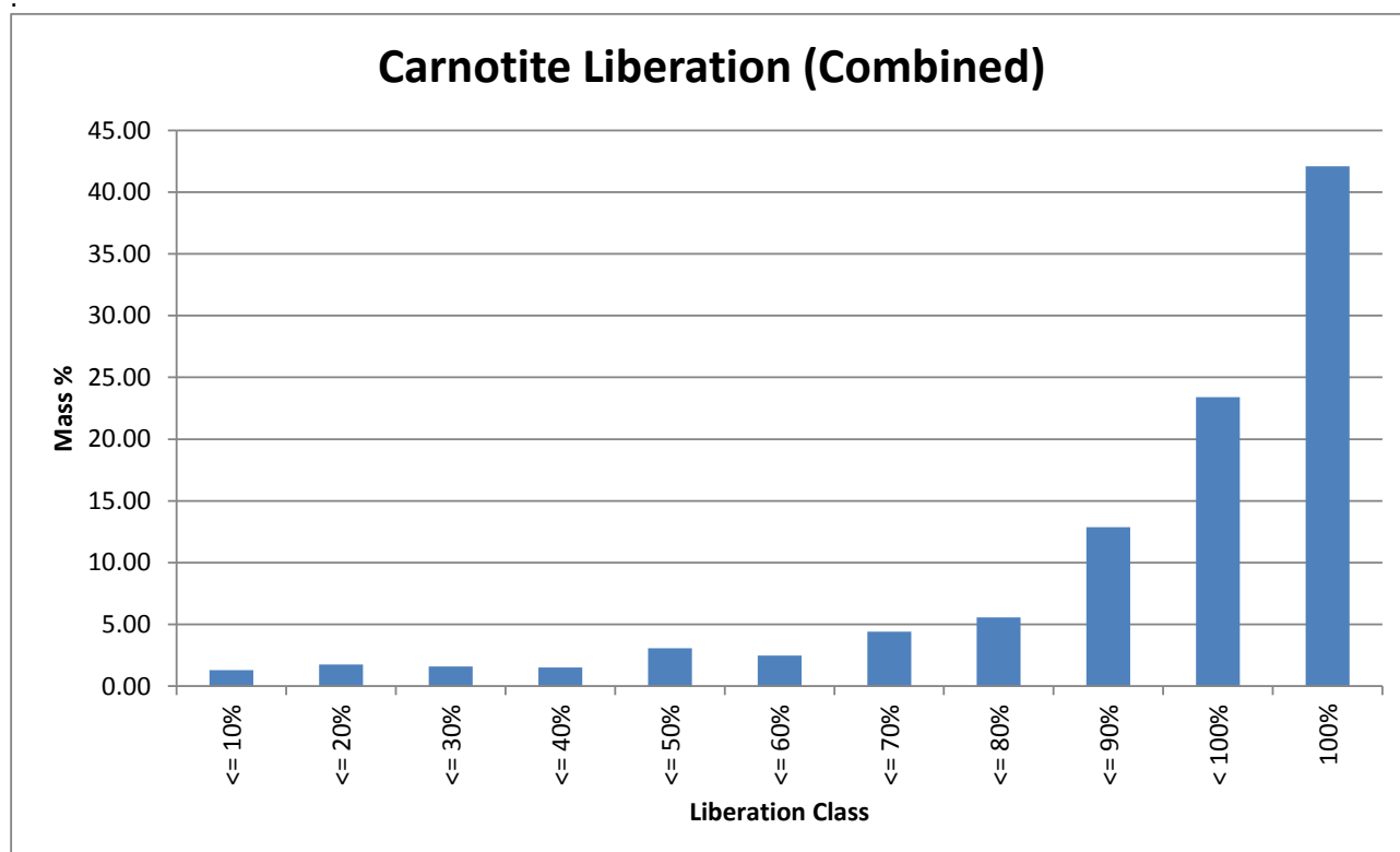
Figure 3. Carnotite Liberation of the Combined -38 \mu and -125/+38 \mu fractions
