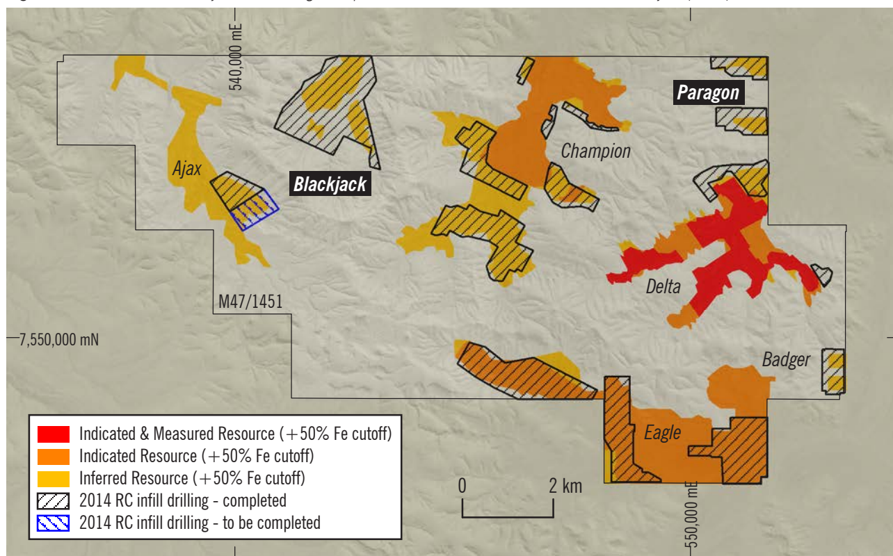
Figure 1 Location of the Blackjack and Paragon deposits within the broader Pilbara Iron Ore Project (PIOP).
