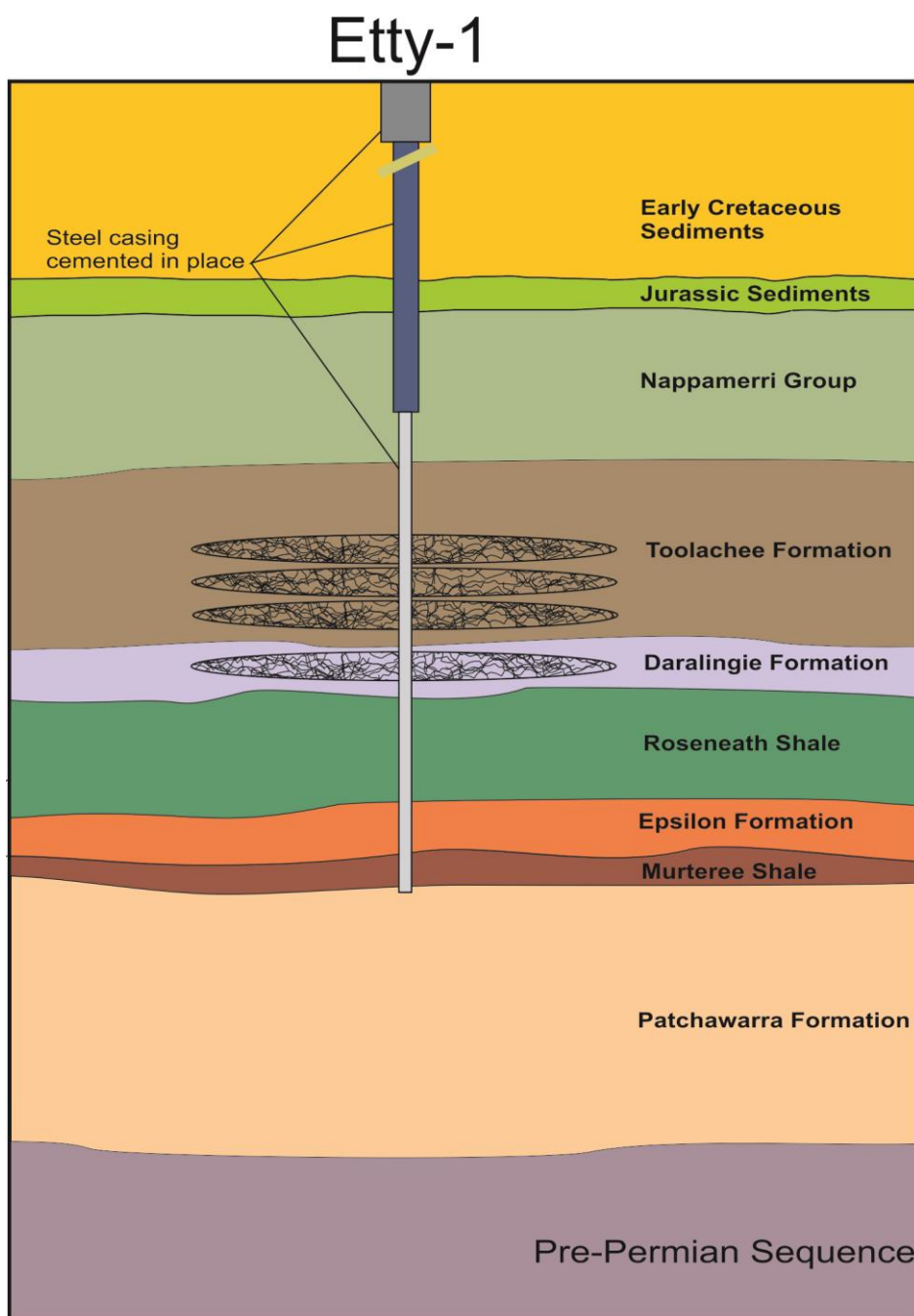
Diagram showing the proposed Toolachee and Daralingie Stimulation zones in Etty-1
