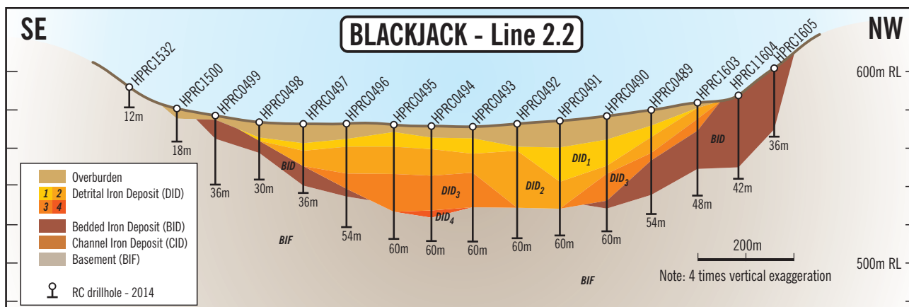
Figure 4 Line 2.2 cross-section through Blackjack deposit.
