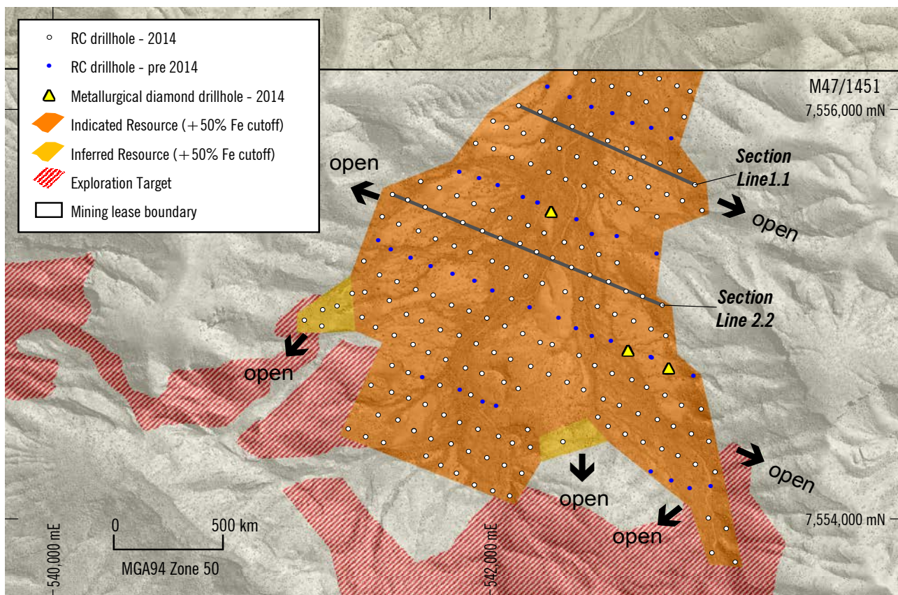
Figure 2 Blackjack deposit drill hole plan.
