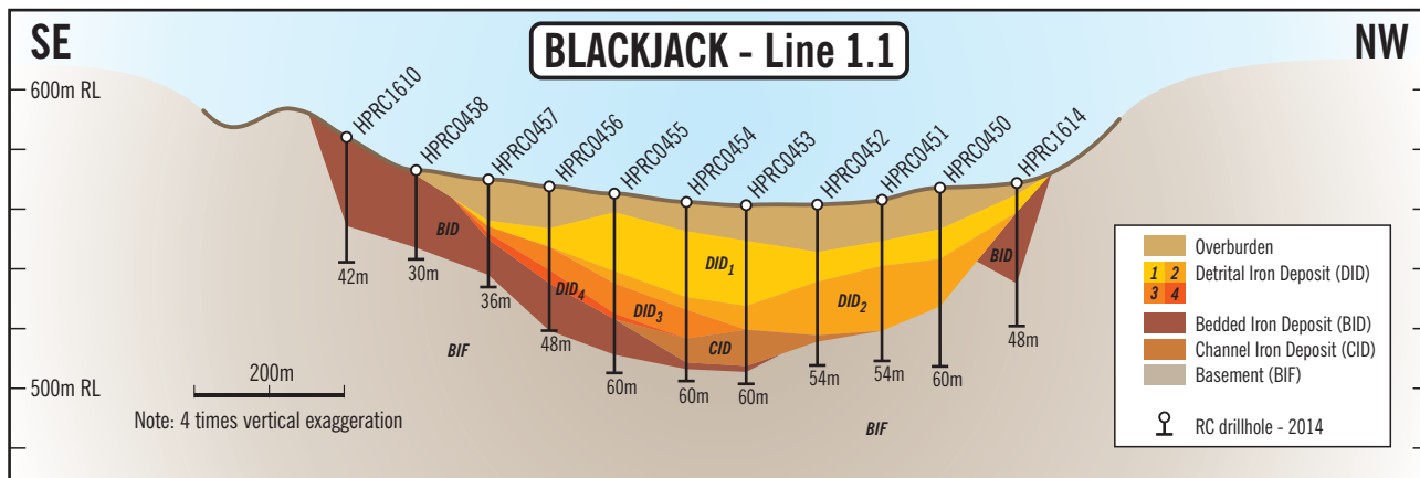
Figure 3 Line 1.1 cross-section through Blackjack deposit.
