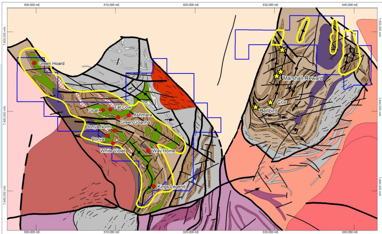
Figure 1: Bonya Project Interpreted Regional Geology (from airborne magnetics) showing prospect locations (red dots) based on prospecting of outcrops
