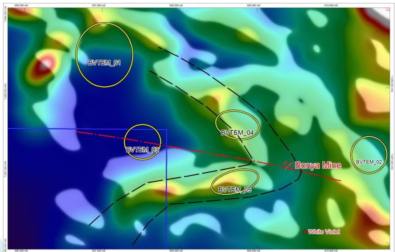
Figure 2: Bonya Mine Area Prospect Locations over Magnetics showing interpreted geology (black lines) and interpreted fold axis (red line)
