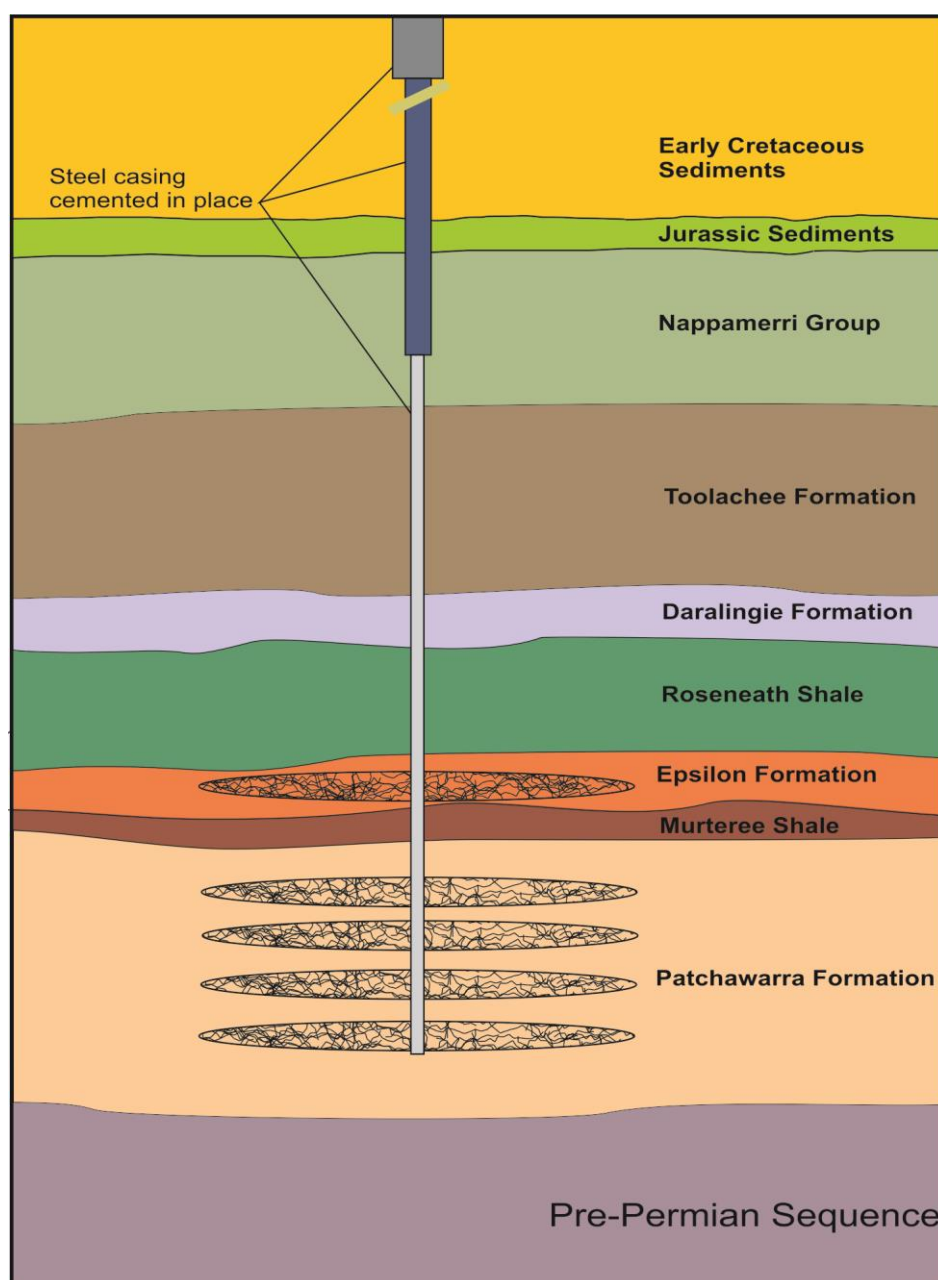
Diagram showing the proposed Patchawarra/Epsilon Stimulation zones in Geoffrey-1
