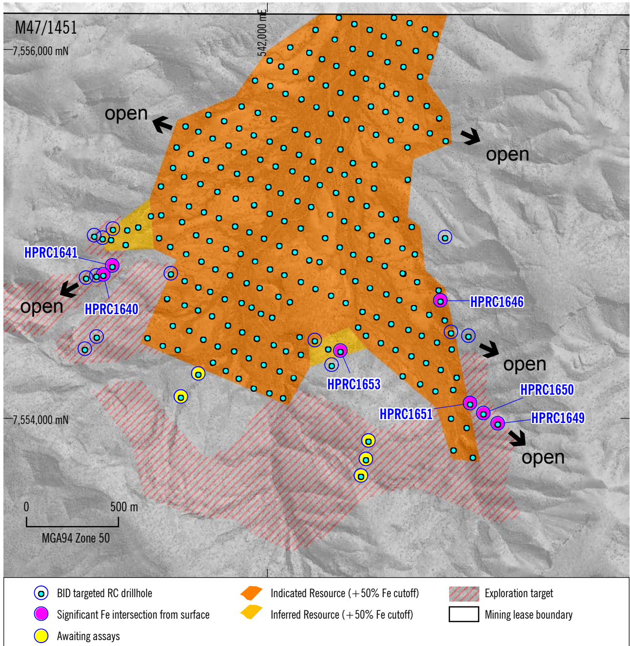
Figure 2 Blackjack Deposit plan highlighting recently completed BID targeted RC drill holes (see Tables 1 and 2).
