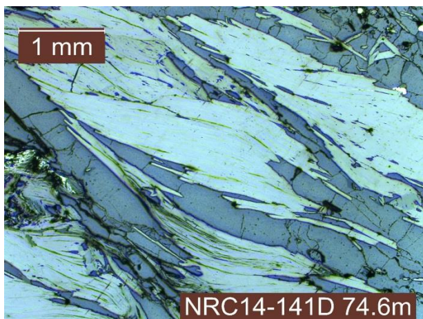
NRC14-141D 74.6m - Graphite sillimanite quartz schist
