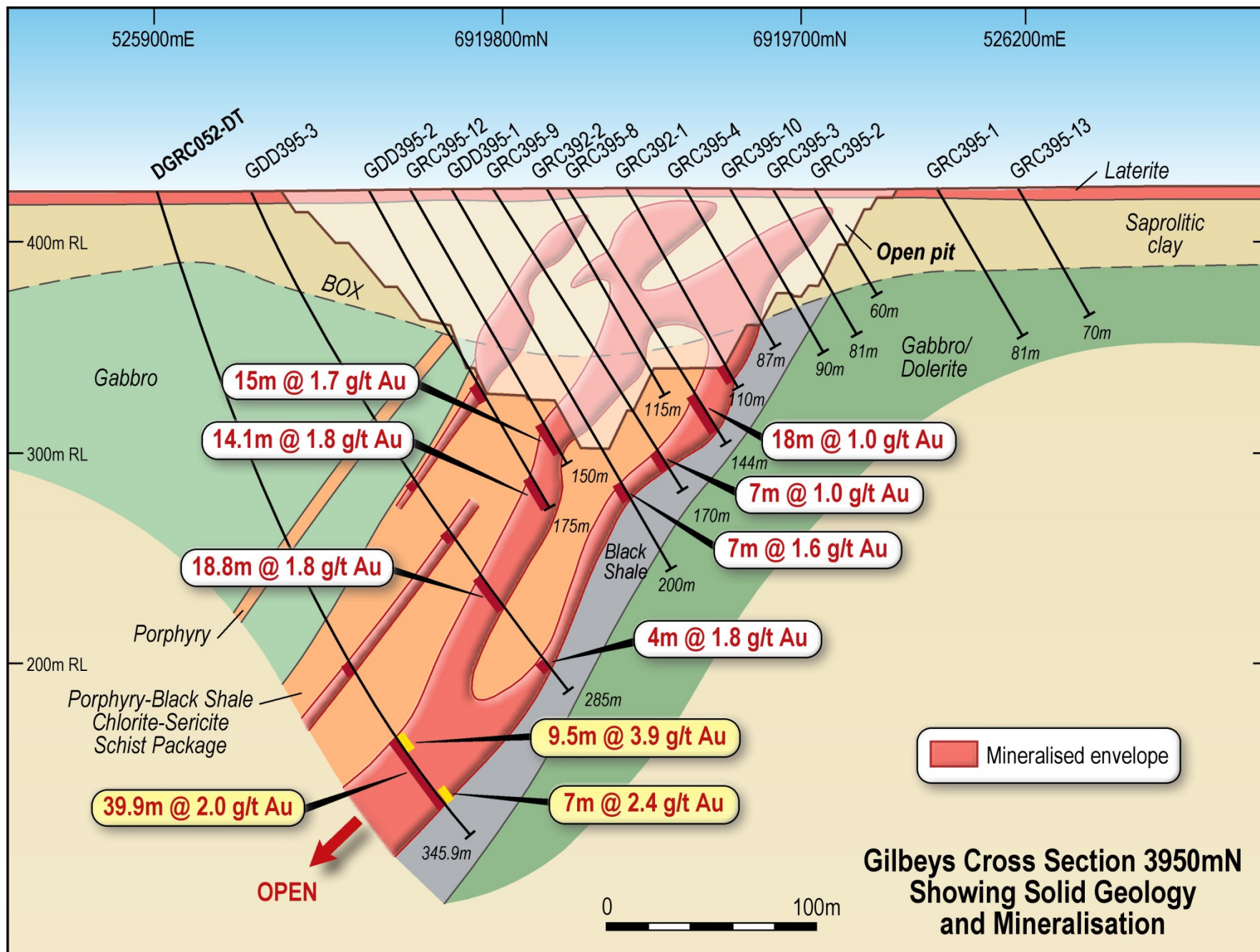
Figure Three: Gilbeys Cross Section 3950m N (new intersections highlighted in yellow)
