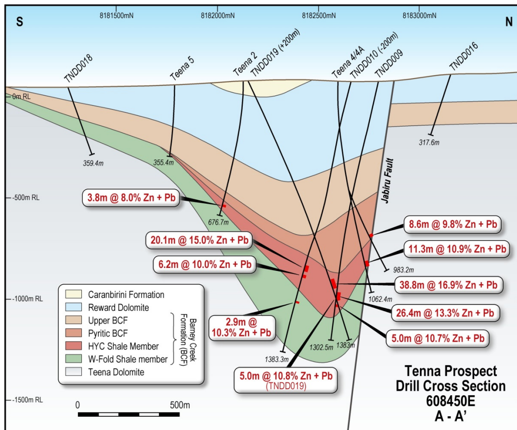
Figure 3: Teena Cross Section A-A'
