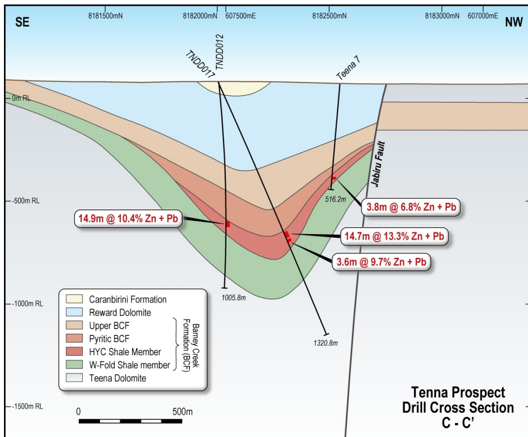
Figure 5: Teena Cross Section C-C'
