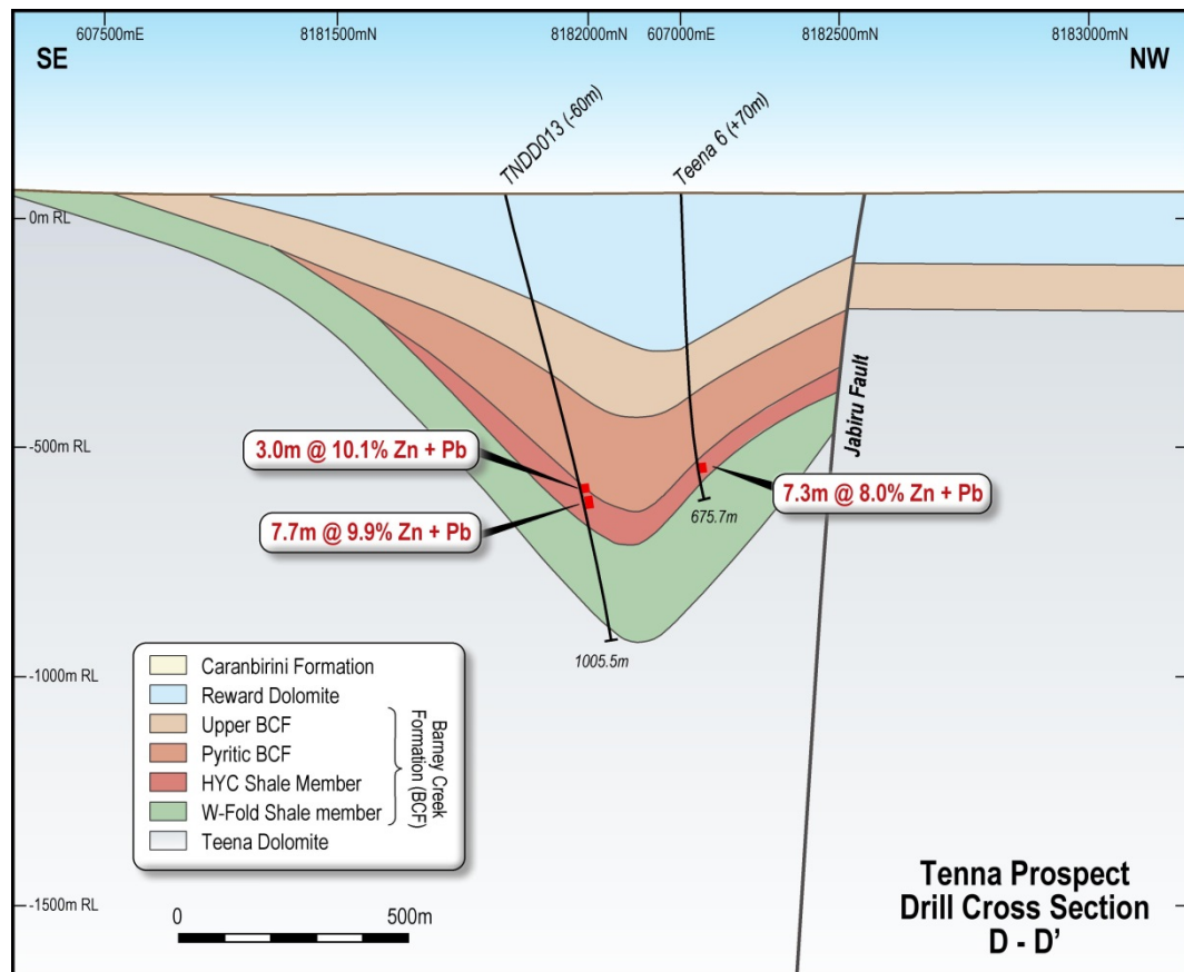
Figure 6: Teena Cross Section D-D'
