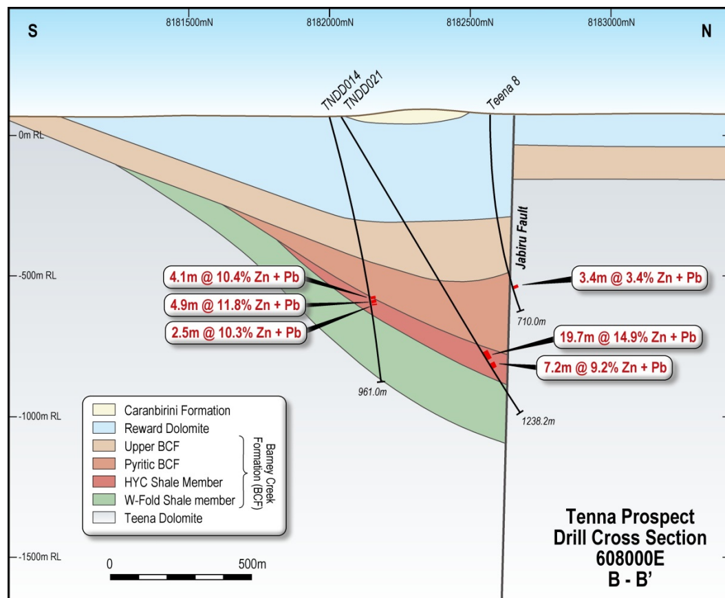
Figure 4: Teena Cross Section B-B'
