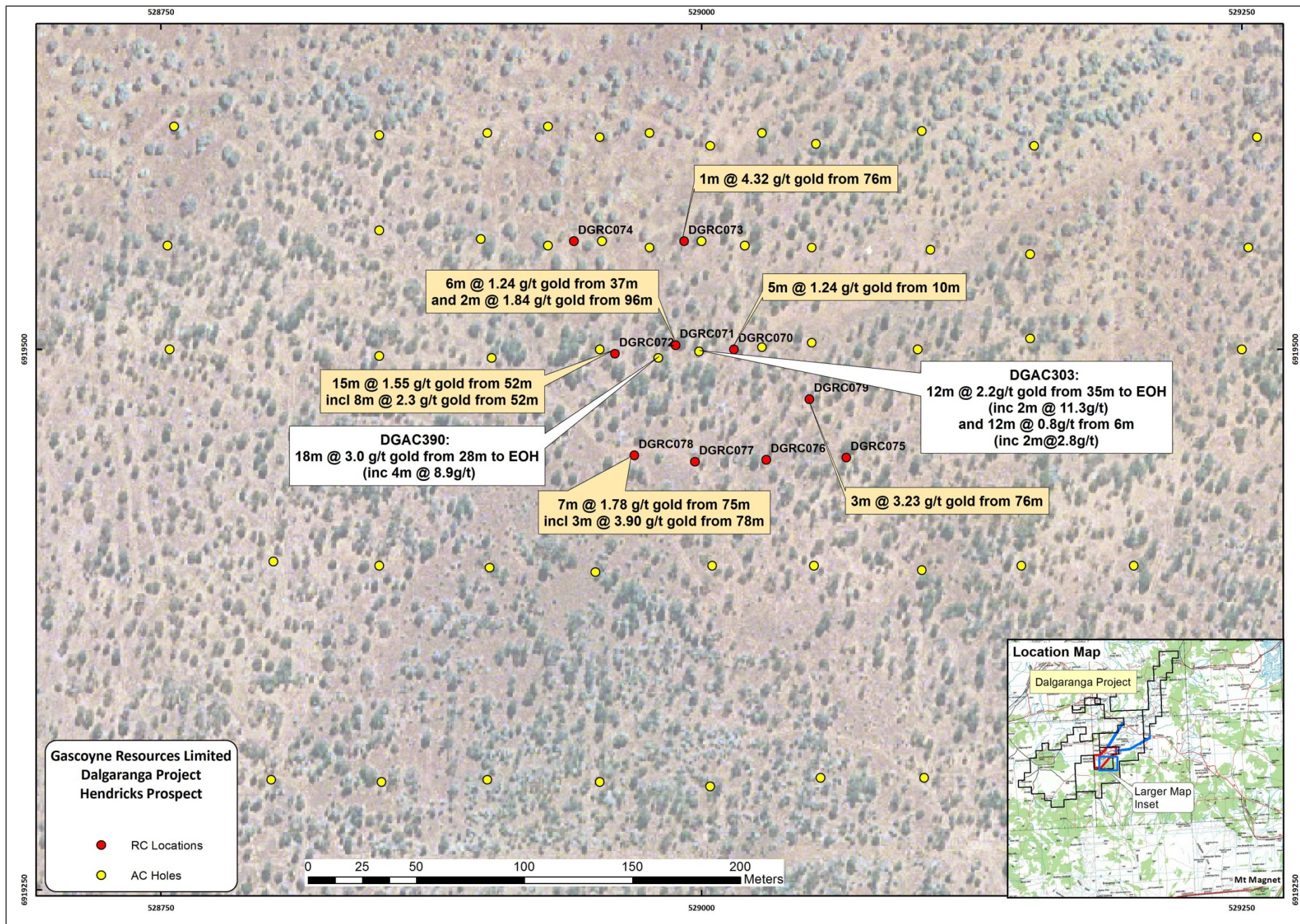
Figure Five: Dalgara Gold Project, Hendricks Prospect Recent RC Drill Intersections
