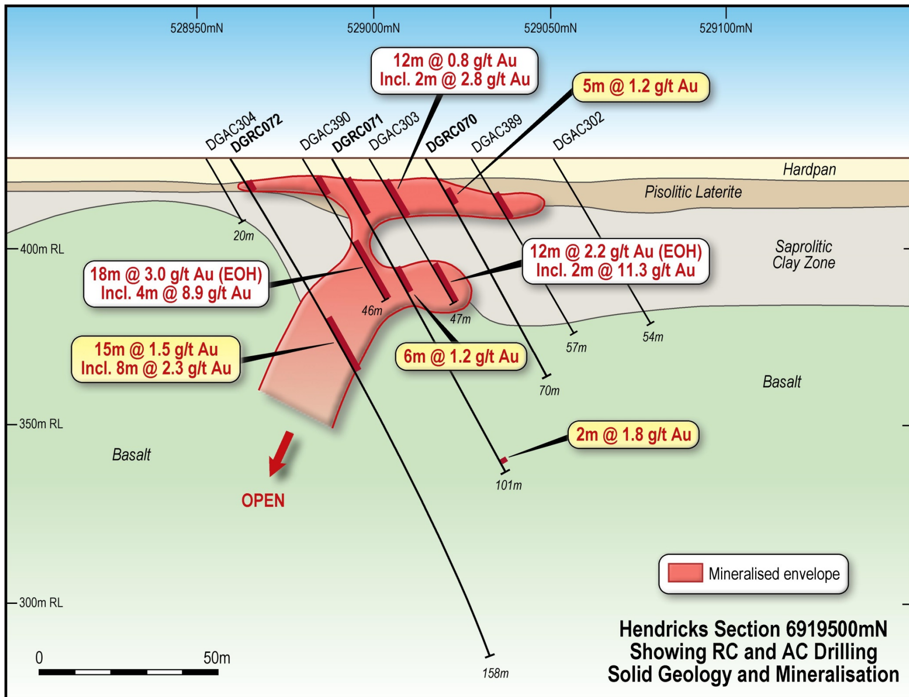
Figure Six: Hendricks Cross Section 6919500 N showing RC and Aircore Drilling Results and Geology
