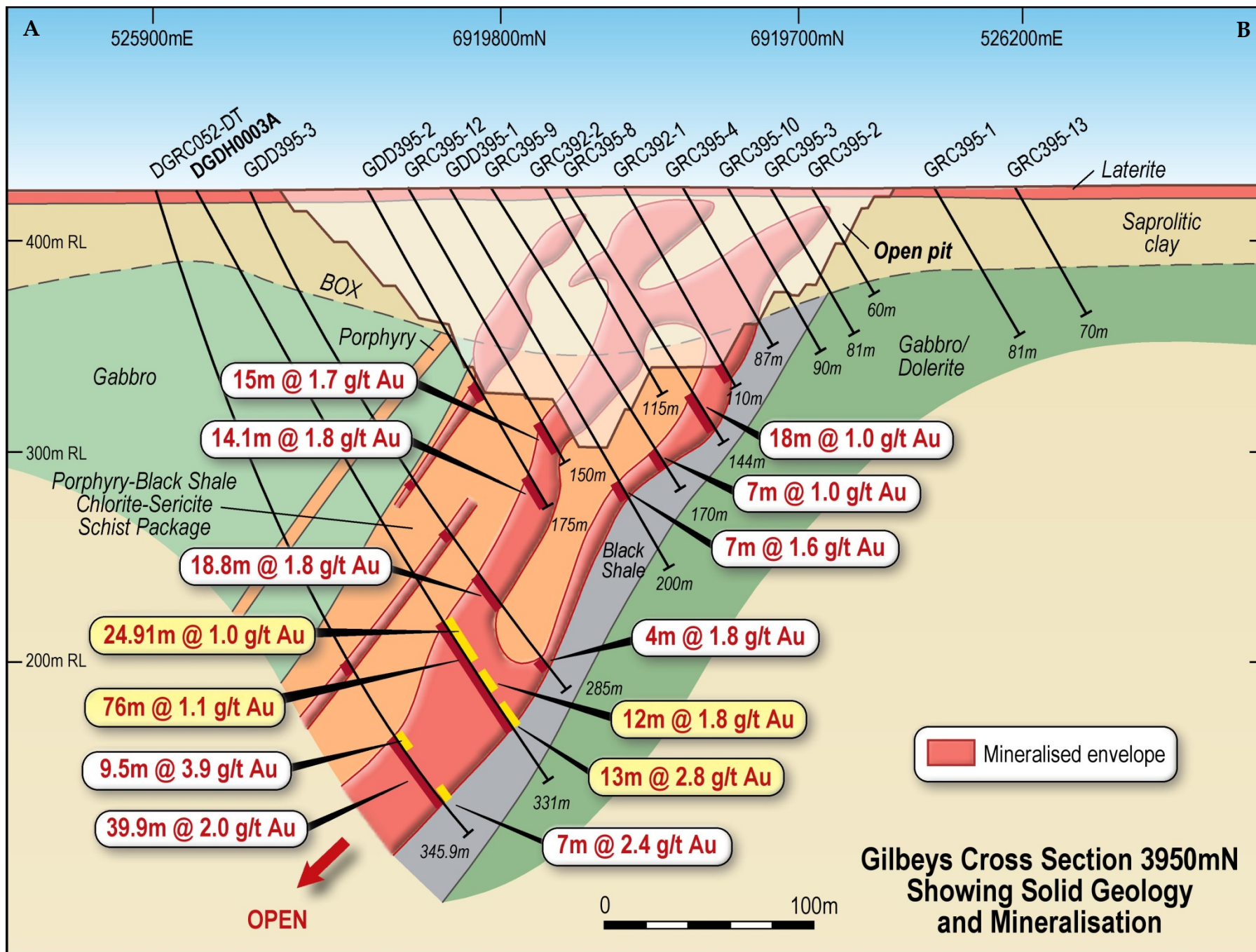
Figure Four: Gilbeys Cross Section 3950 N showing Recent Diamond Core Drilling Results and Geology
