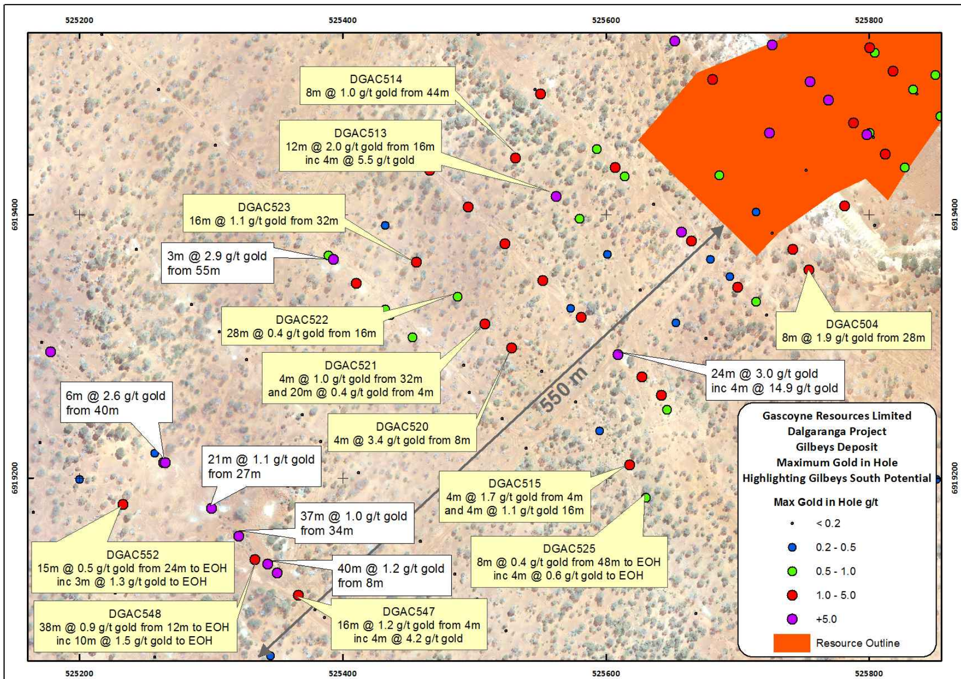
Figure Four: Gilbeys South Maximum gold in Hole and current resource outline highlighting potential for growth to the South West (new intersections highlighted in yellow, historical significant intersections in white)
