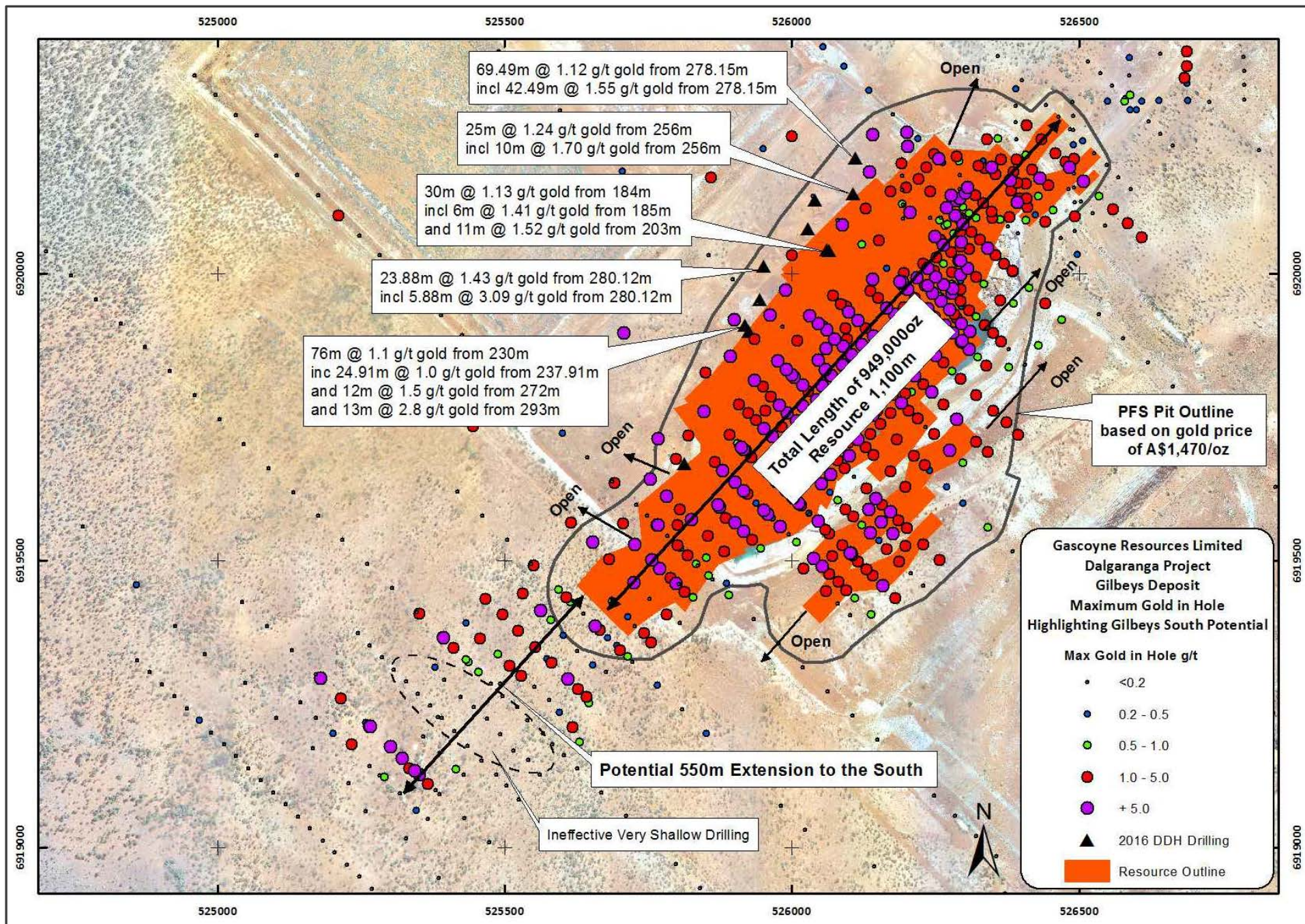
Figure Three: Gilbeys Deposit Maximum gold in Hole, resource outline and conceptual PFS pit outline highlighting potential for growth to the South West
