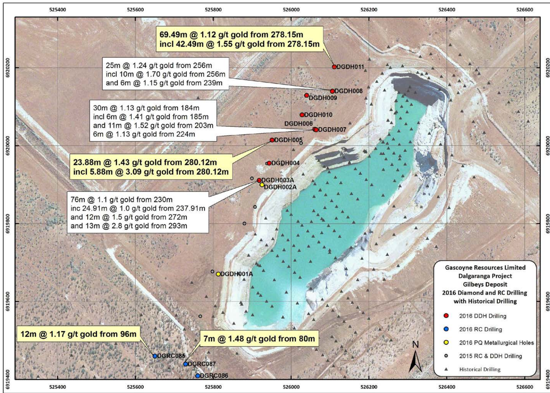
Figure Five: Dalgaranga Gold Project, Gilbeys Deposit Recent RC and Diamond Core Drill Intersections
