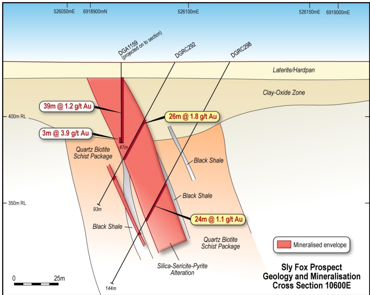
Figure Five: Sly Fox Cross Section 10600E
