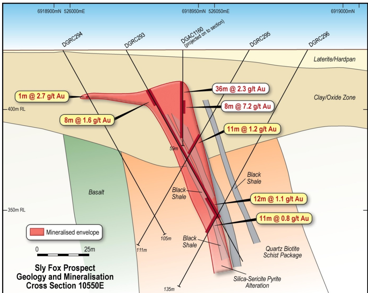
Figure Six: Sly Fox Cross Section 10550E
