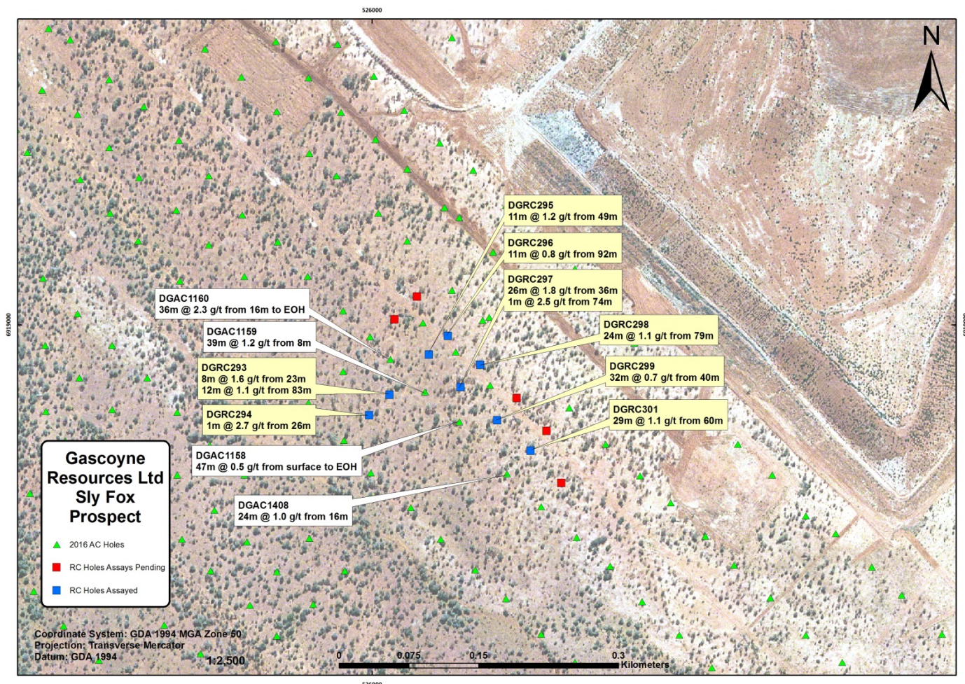
Figure Three: Dalgara Gold Project, Sly Fox – Recent RC Drill Intersections
