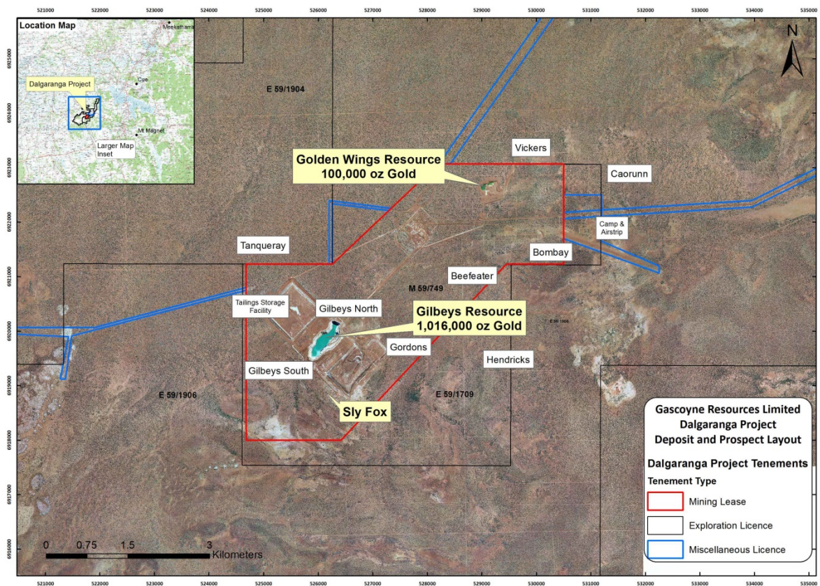
Figure Two: Dalgarranga Gold Project Deposit and Prospect Layout
