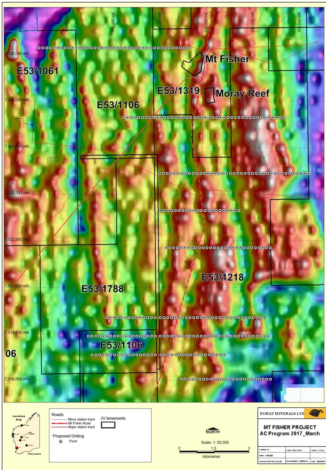
Figure 2: Mt Fisher Planned Aircore Drilling
