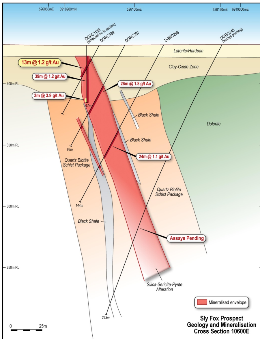
Figure Five: Sly Fox Cross Section 10600E
