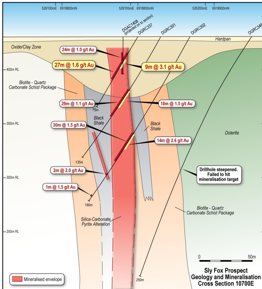
Figure Seven: Sly Fox Cross Section 10700E
