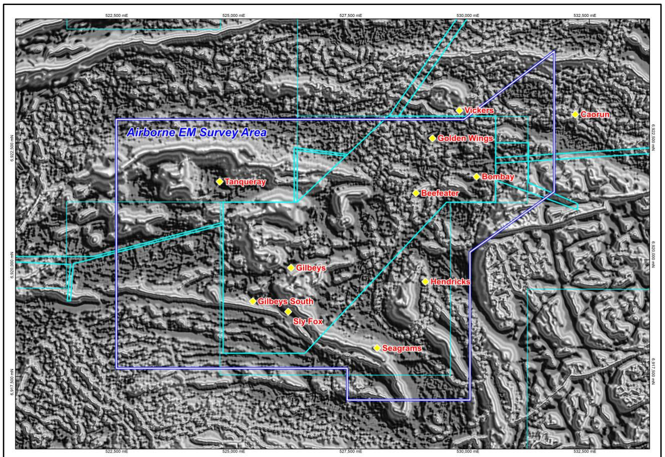
Figure Eight: Helicopter Electromagnetic Survey Area over Aeromagnetic Image (dark blue survey outline, tenements outlined in light blue)
