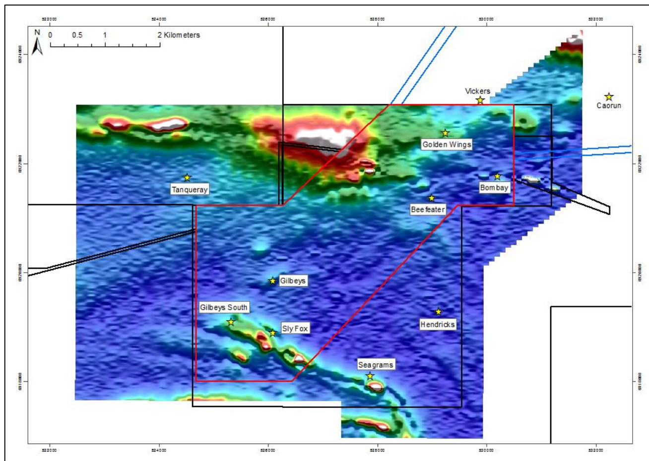
Figure Nine: Helicopter Electromagnetic Survey – Late Time (Bedrock) Response (Red and White zones represent more conductive horizons)
