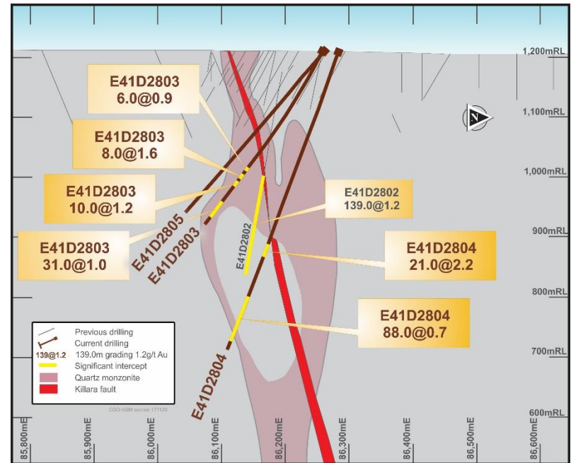
E41 West oblique section showing recent drill hole results
