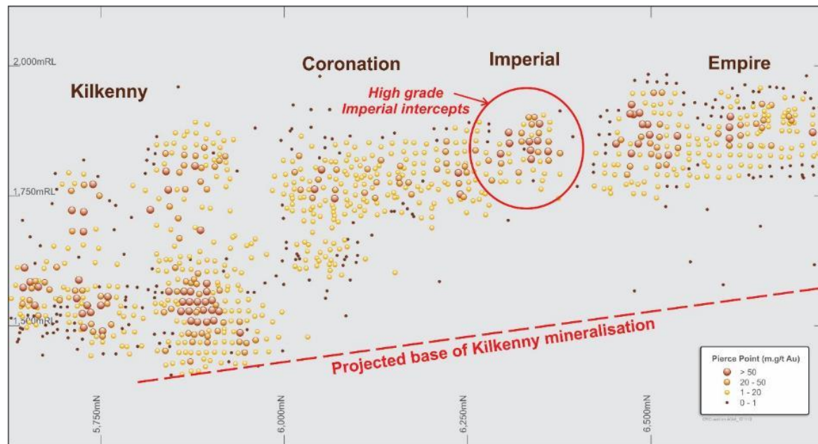
Long section illustrating location of the new Imperial shoot defined between the Coronation and Empire ore bodies
