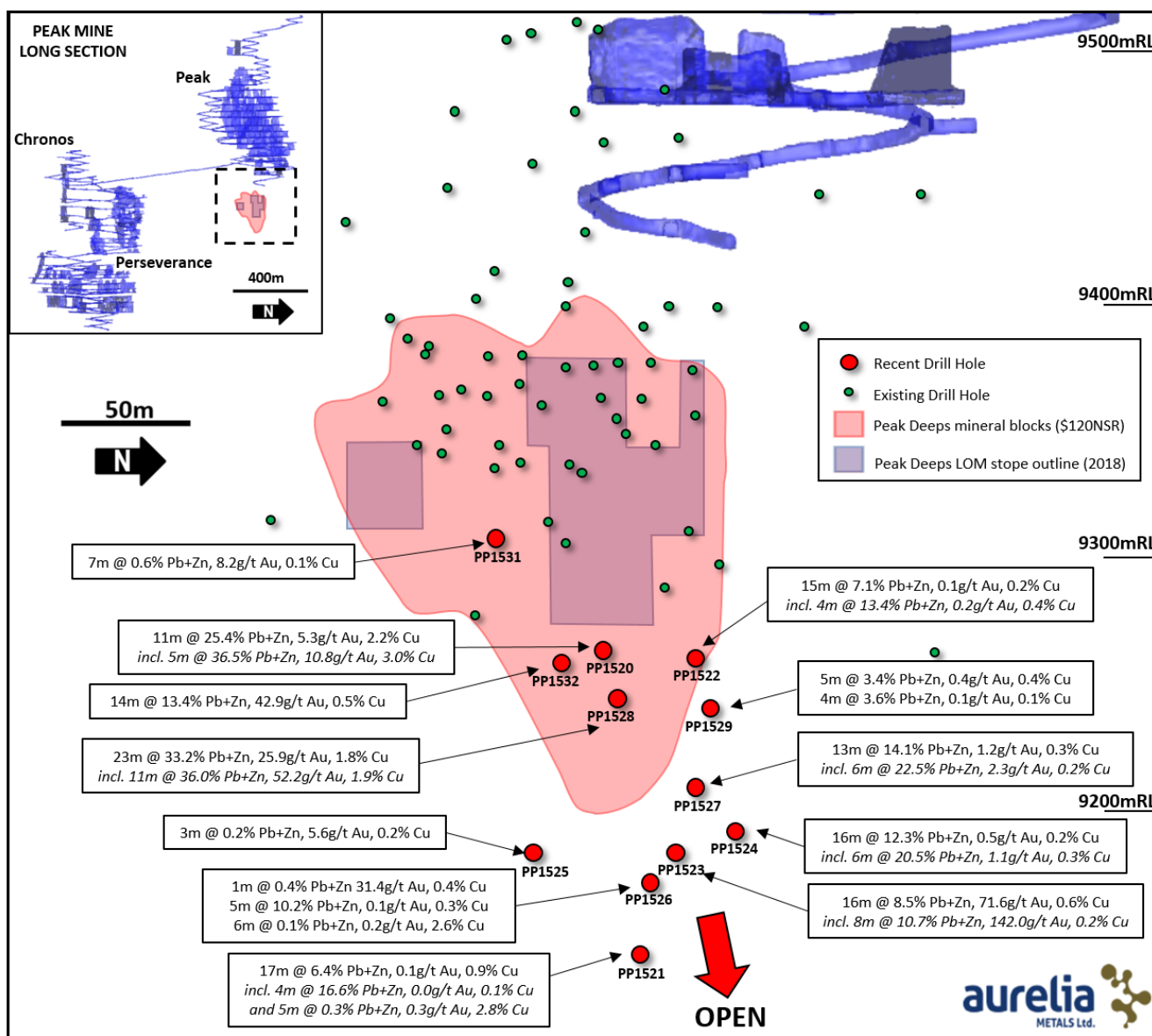
Figure 1. Long section showing recent and historic drilling at Peak Deeps, including significant intercepts.
