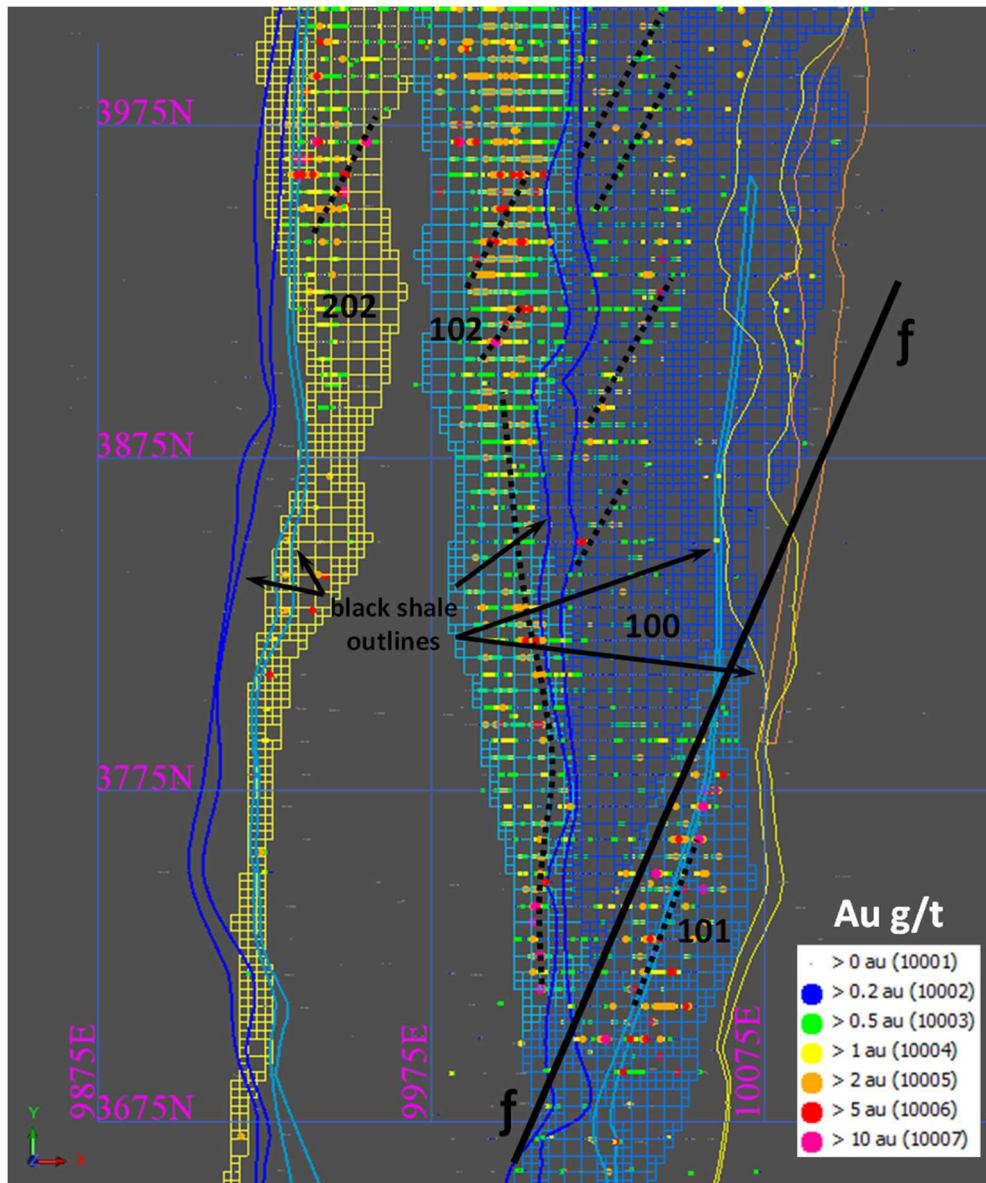
Figure 4: Plan cross-section view at 355mRL – estimation domains represented by variably coloured blocks. Key lithological and structural features are shown, including mineralisation trends oblique to main zone trend (stippled lines).
