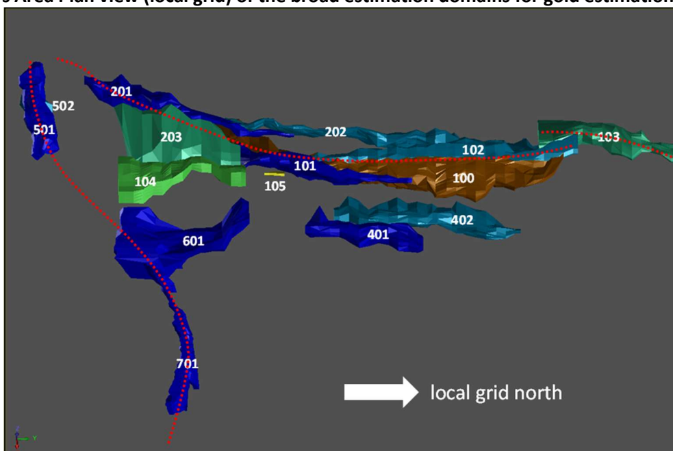
Figure 2: Gilbey's Area Plan view (local grid) of the broad estimation domains for gold estimation.
