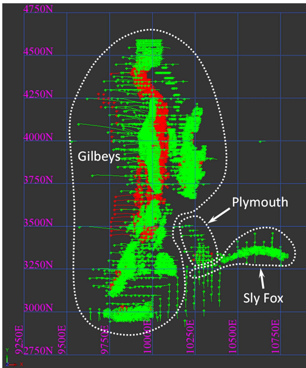
Figure 11: Plan view, in local grid, of holes used during the previous and update gold grade estimates. Green = holes used both previously and in this update; red = new holes not used previously but included in update estimate.
