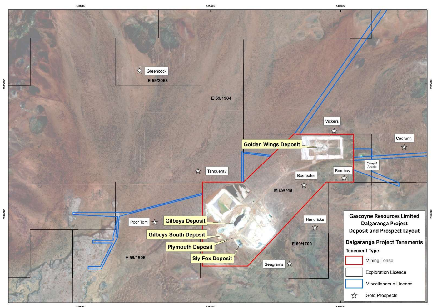
Figure 18: Dalgara Gold Project Deposit and Prospect Layout
