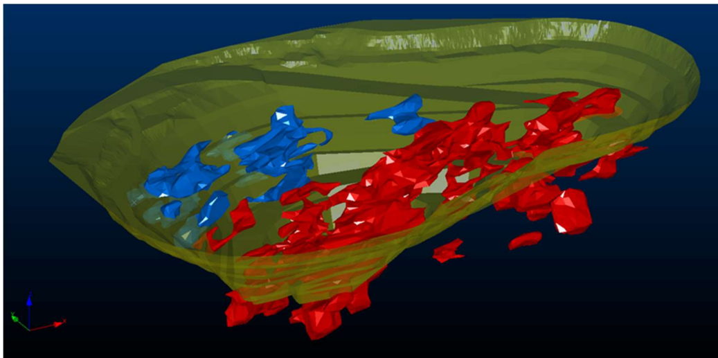
Figure 16: Golden Wings 0.25 gold grade indicator - 35% probability iso-surface
