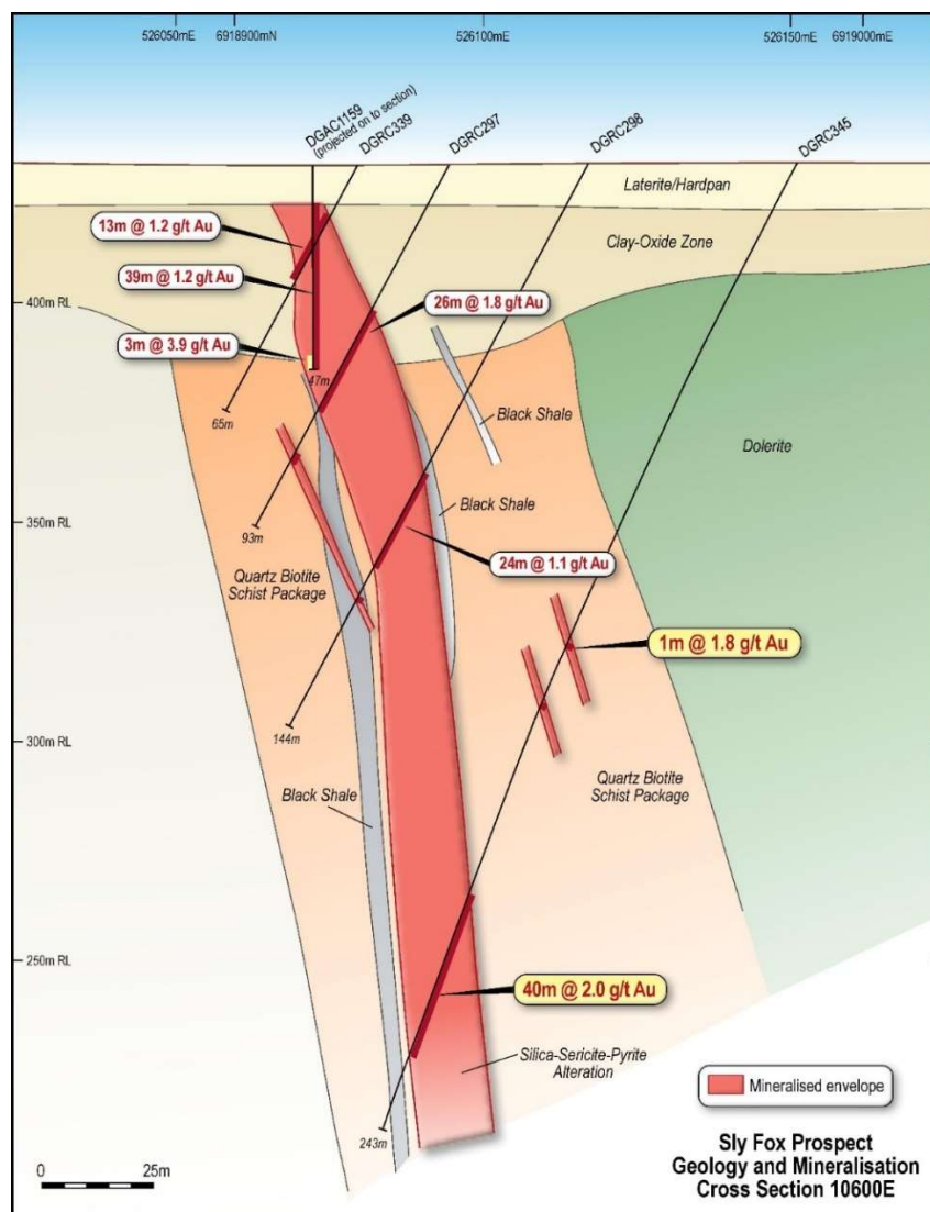
Figure 10: Cross-section interpretation of the Sly Fox deposit at local grid 10600mE, looking westwards
