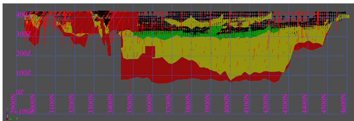
Figure 14: Dalgara classification long section view looking towards the west (local grid) – depleted, showing non-halo domains. Black traces = GC holes; Red traces = RDV holes.
