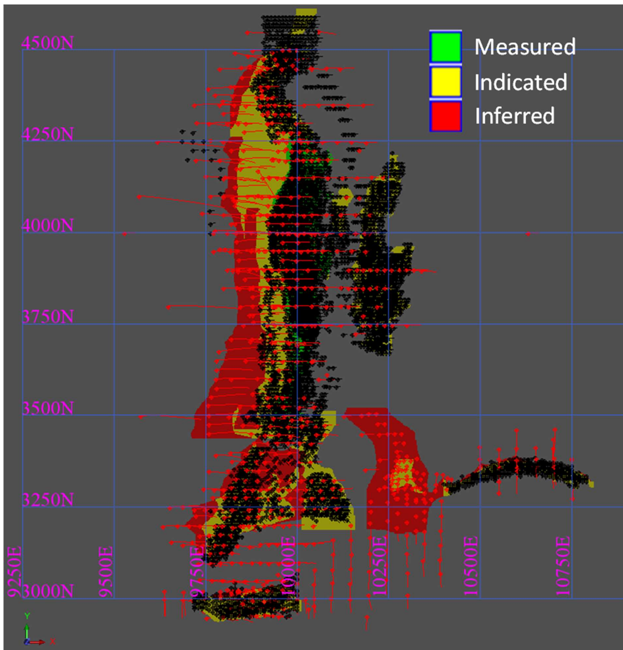
Figure 12: Dalgaranga classification plan view – depleted, showing non-halo domains. Black traces = GC holes; Red traces = RDV holes.
