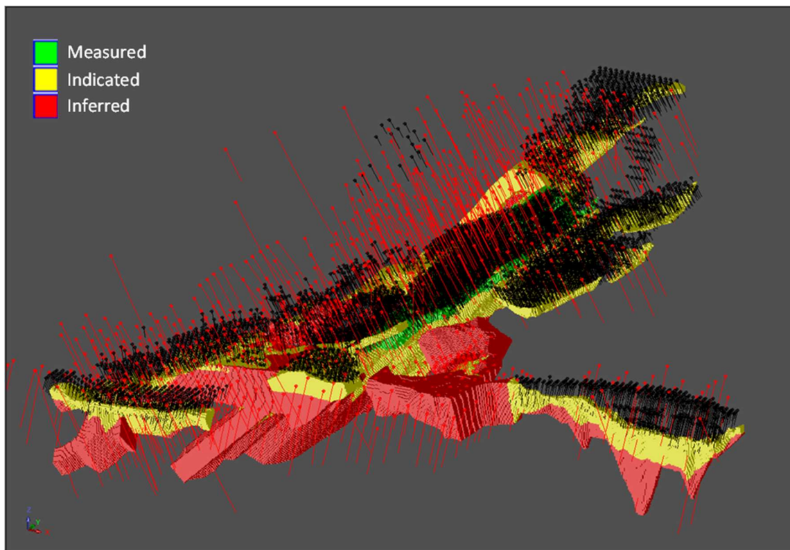
Figure 13: Dalgara classification isometric view looking towards the northwest (local grid) – depleted, showing non-halo domains. Black traces = GC holes; Red traces = RDV holes.
