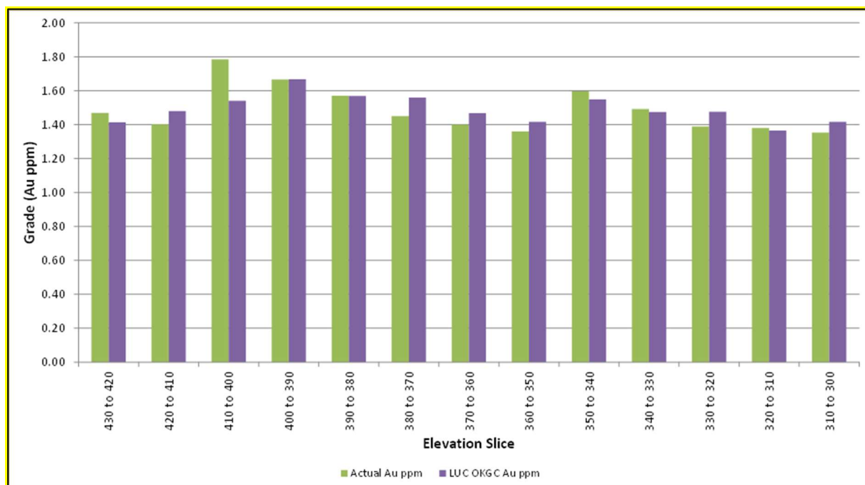
Figure 6: Gold grade comparison by elevation slice – Equigold Actuals vs LUC OK GC Model
