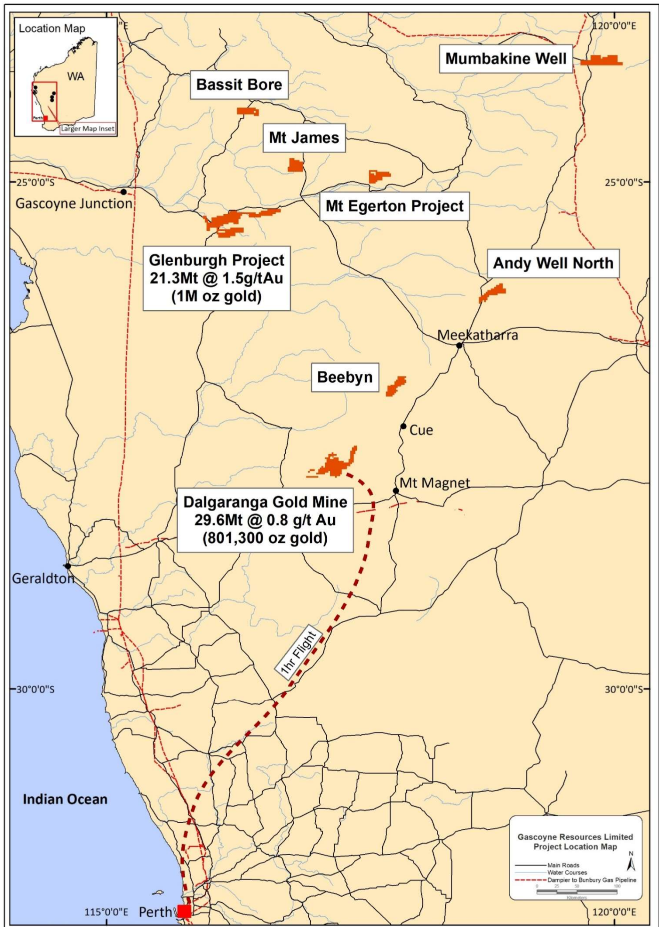
Figure 17: Project Locations in the Gascoyne and Murchison Regions
