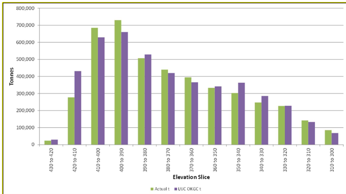
Figure 5: Tonnes comparison by elevation slice – Equigold Actuals vs LUC OK GC Model
