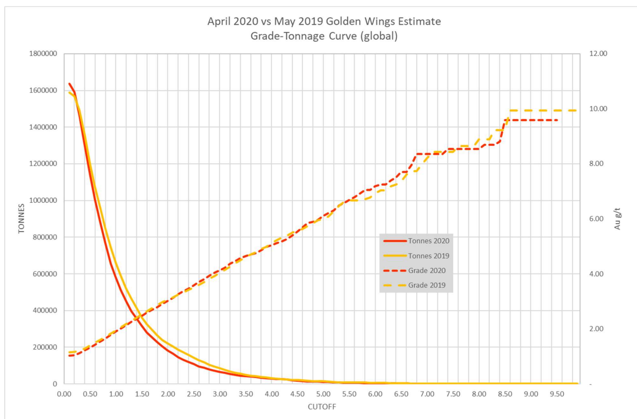
Figure:8 2020 Golden Wings 2020 Estimate vs 2019 Estimate (grade-tonnage curves)
