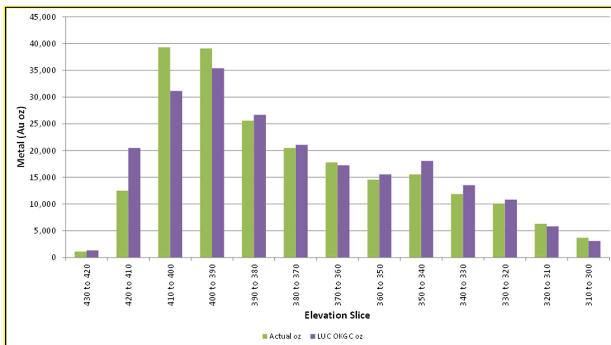
Figure 7: Gold ounces comparison by elevation slice – Equigold Actuals vs LUC OK GC Model
