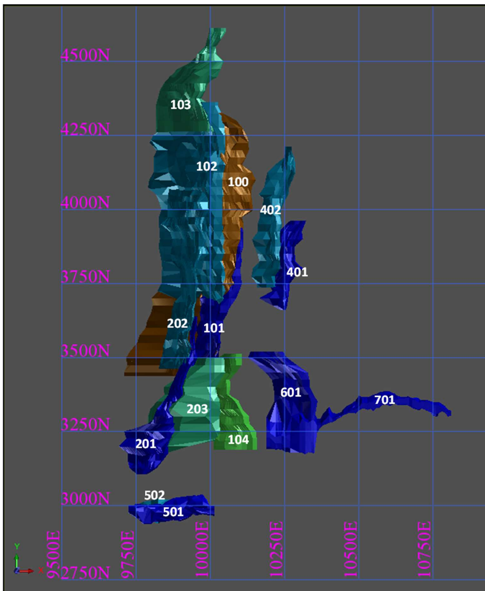
Figure 2: Gilbey's Area Plan view (local grid) of the broad estimation domains for gold estimation.
