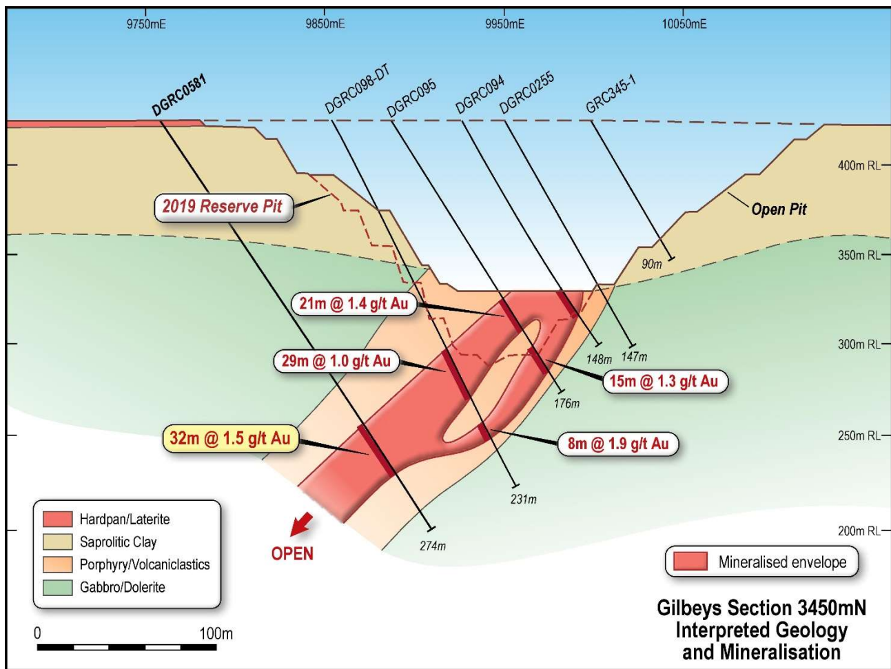
Figure 9: Cross-section interpretation of the Gilbey's deposit at local grid 3450mN, looking northwards
