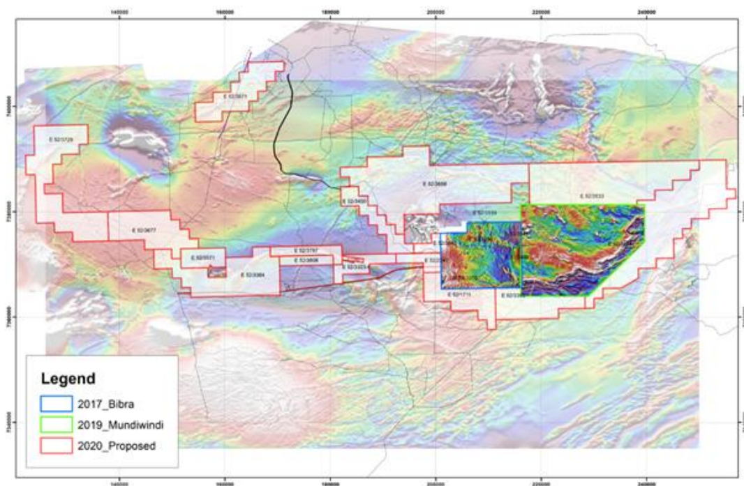
Figure 4: Aeromagnetic survey
