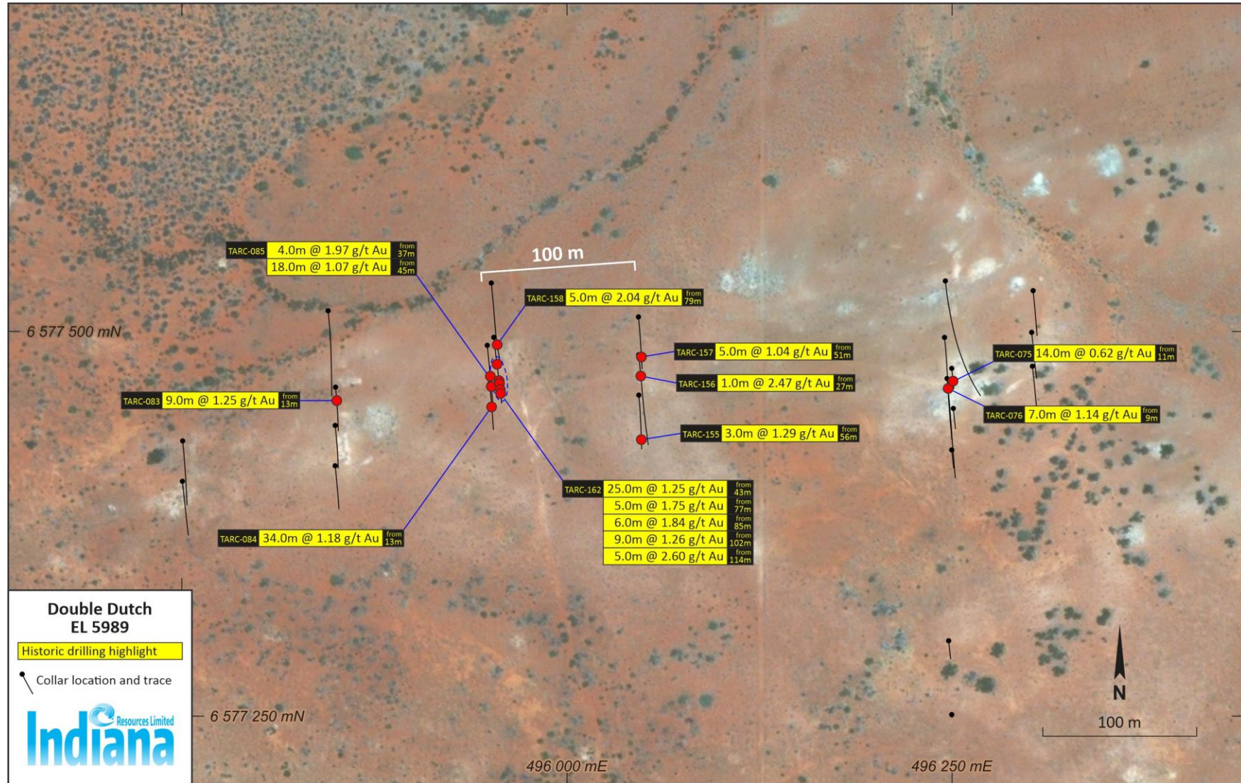
Figure 4: Significant Drilling Results – Double Dutch Prospect
