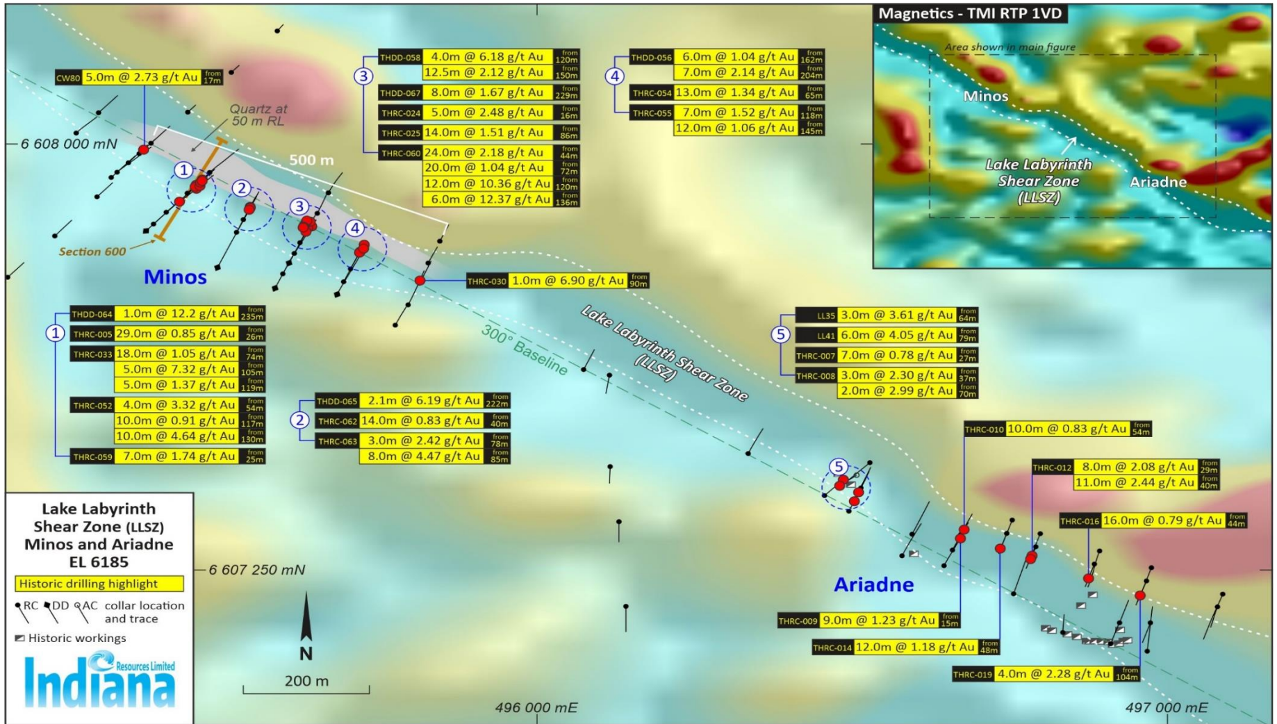
Figure 3: Lake Labyrinth Significant Historic Drilling Results – Minos and Ariadne Prospects sowing Minos 600 Section Line
