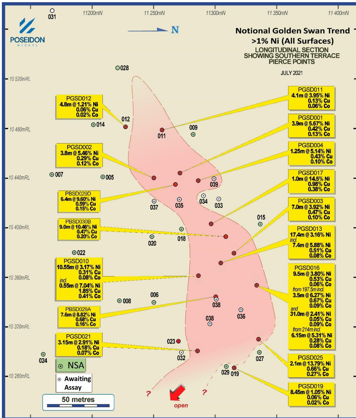
Figure 1: SIMPLIFIED GOLDEN SWAN LONG SECTION SHOWING CURRENT PIERCE POINTS AND SIGNIFICANT DRILL RESULTS
