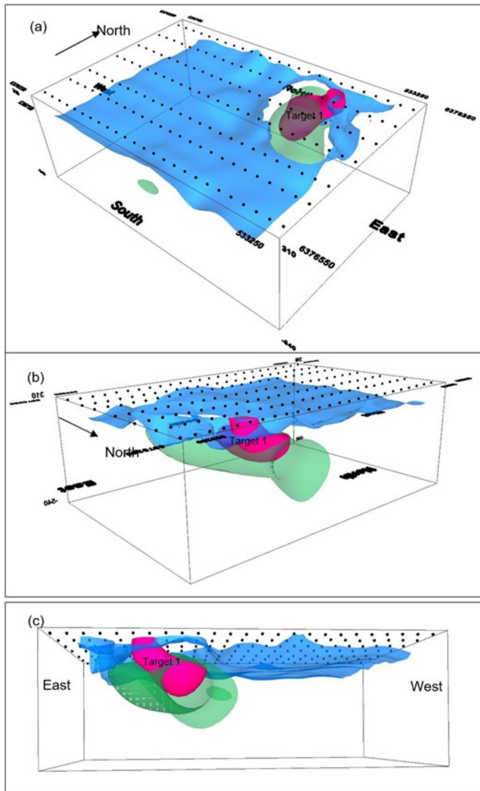
Figure 11: Perspective views of iso-shells created from the Flemington Induced Polarisation (IP) 3D inversion models. Chargeability shell (14 mV/V) shown in pink. Low resistivity (100 \Omega m) surface layer shown in blue and higher resistivity (2000 \Omega m.m) zone in green. Views are from (a) the south-east, (b) the north-east, and (c) from the north and below surface 94 .
