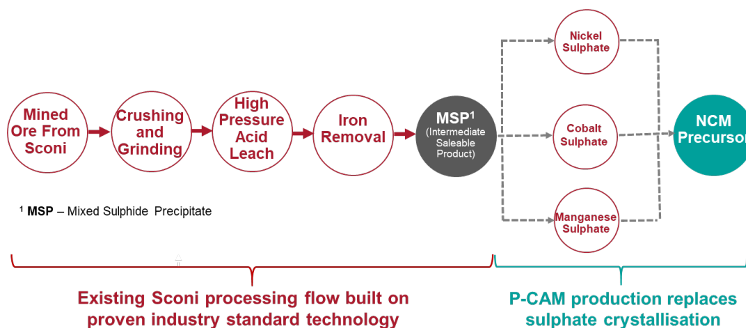
Figure 2: Australian Mines Sconi Project processing flowsheet, substituting precursor cathode active material (P-CAM) production for the sulphate crystallisation stage.
