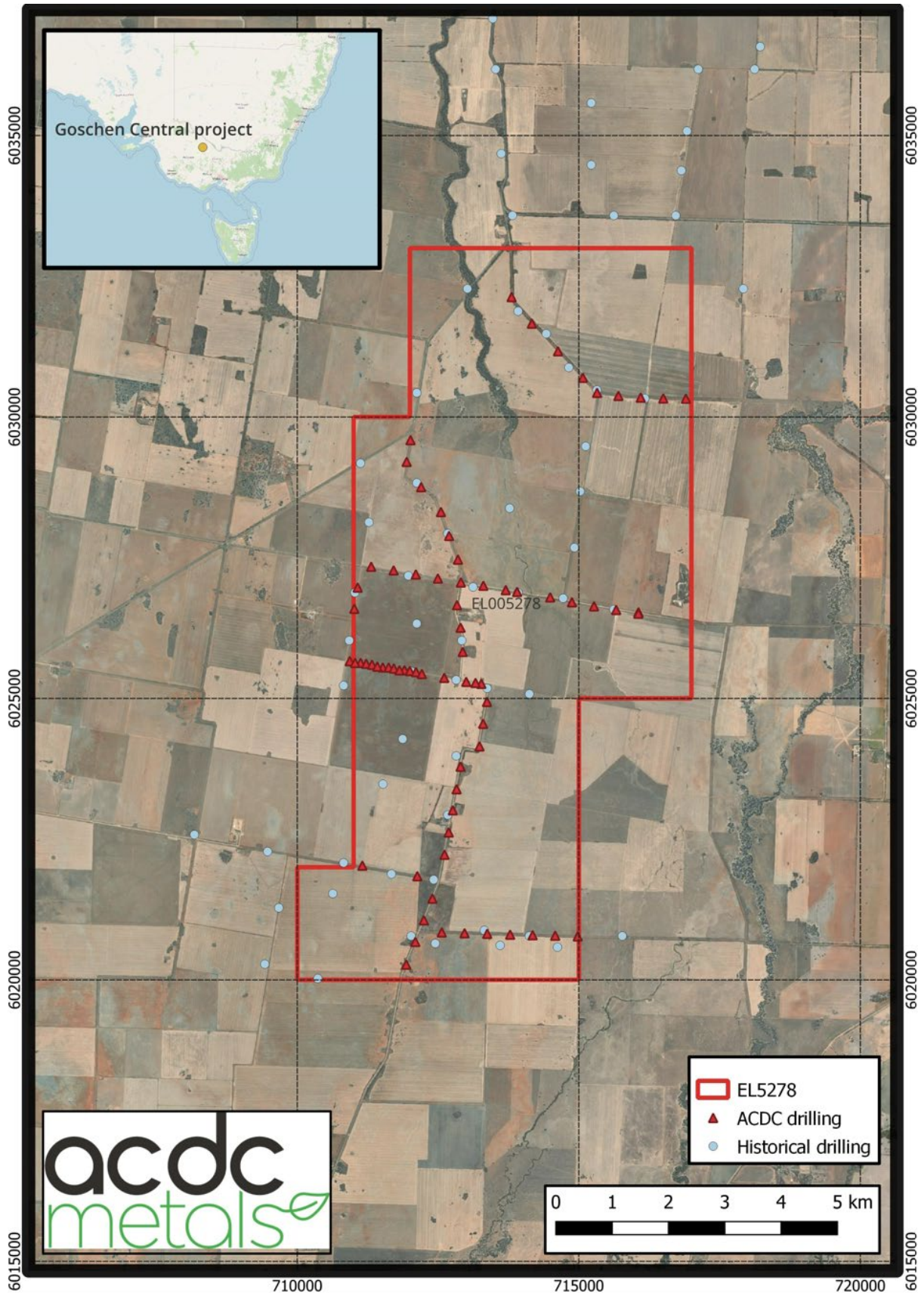
Figure 1 EL5278 Drill plan
