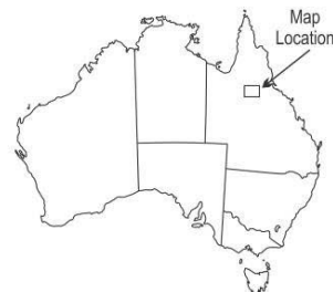
Figure 2. ActivEX Limited Gilberton Gold Project regional geology, tenements, prospect and rock chips thematically mapped by Au content.
