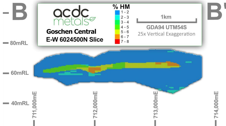
Figure 3 Section view 6024000N, Surface at ~95mRL, see figure 1.
