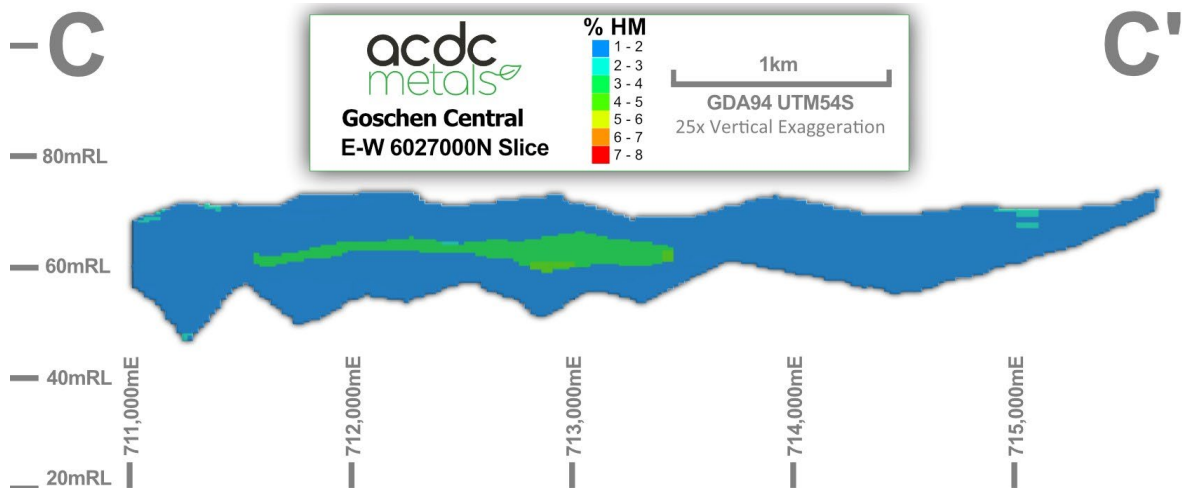
Figure 4 -Section view 6027000N, Surface at ~95mRL, see figure 1.
