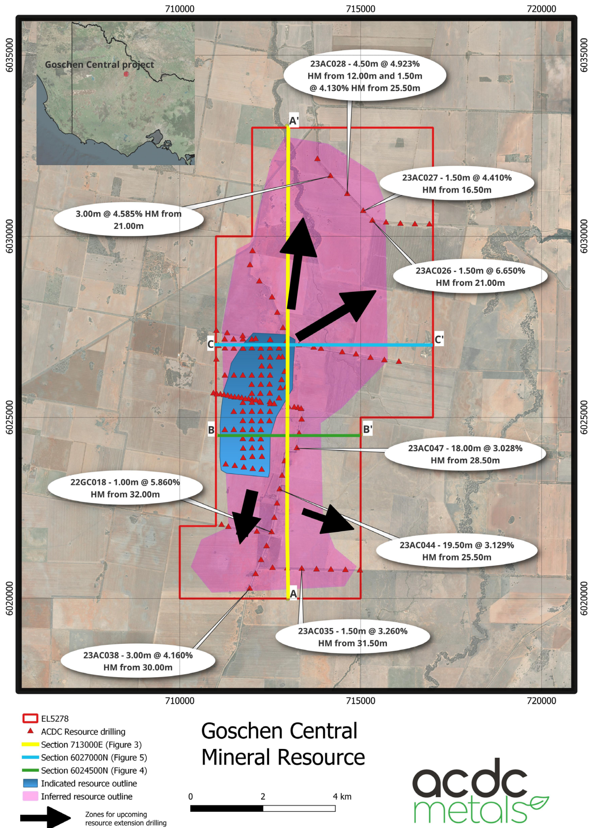
Figure 1 –Resource Outlines and zones of resource extension for upcoming resource extension drilling.
