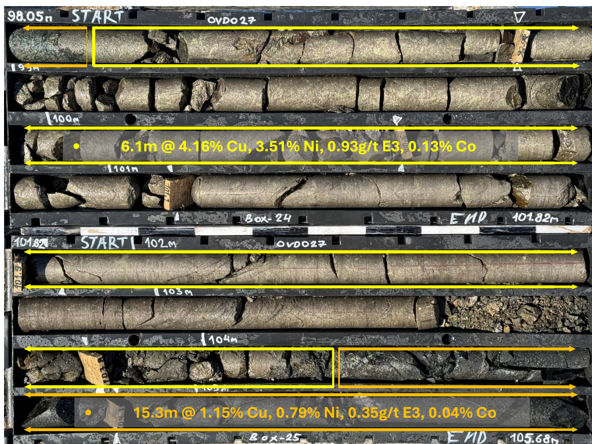
Photo 2. Massive sulphide intersection in drillhole OVD027
